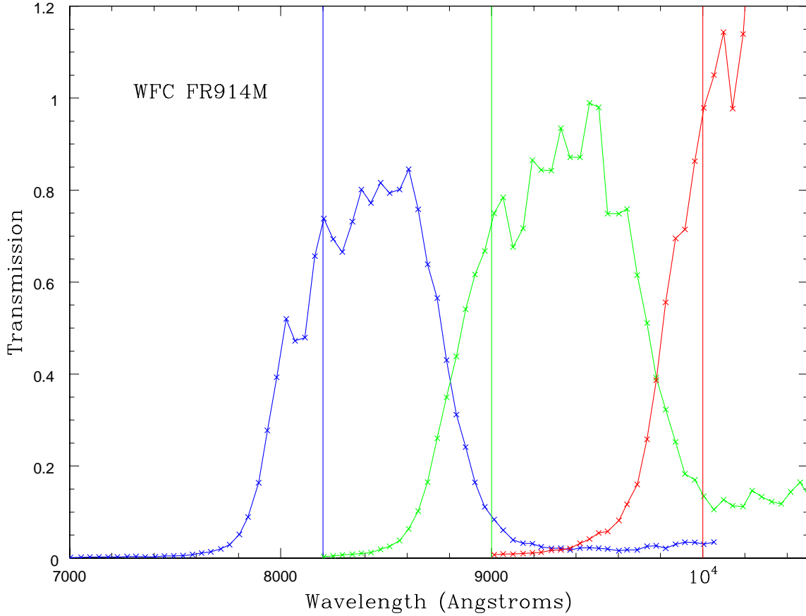
Fig. 6.— Plots of the measured transmission of the ramp filter FR914M on the WFC, set at three central wavelengths: 8200, 9000 and 10,000 Å. The transmission of greater than 100% for the setting of 10,000 Å is most likely caused by an extrapolation of the stellar spectrum beyond 9200 Å, combined with a poor understanding of the flat-field of the grism below 10,000 Å.
