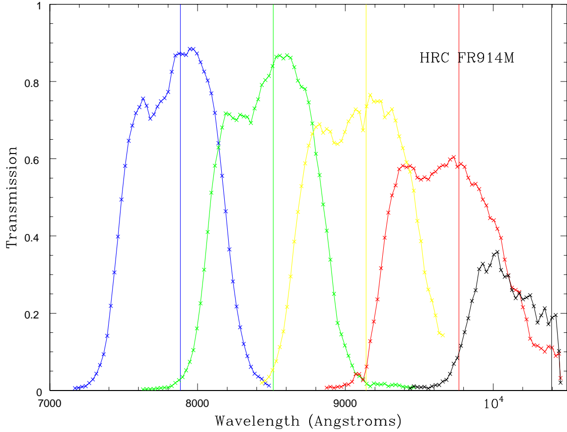
Fig. 2.— Plots of the measured transmission of the ramp filter FR914M on the HRC, set at five central wavelengths: 7884, 8512, 9140, 9768 and 10396 Å. These wavelengths are shown by the vertical lines. The long-wavelength end of the spectrum of the third setting, with expected central wavelength 9140 Å, was corrupted by a cosmic-ray, and is not shown. These observations were taken as part of CAL 9671.
