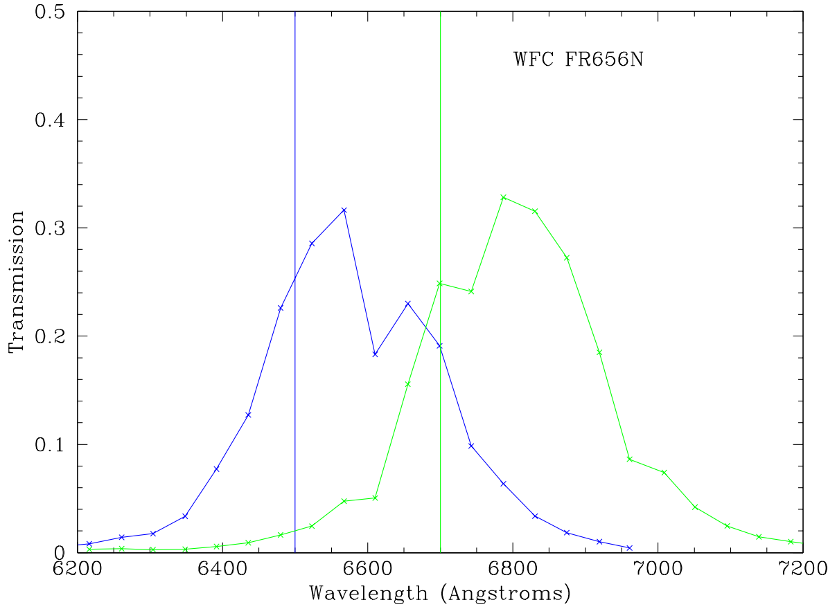
Fig. 5.— Plots of the measured transmission of the ramp filter FR656N on the WFC, set at two central wavelengths: 6500 and 6700 Å, shown by the vertical lines.
