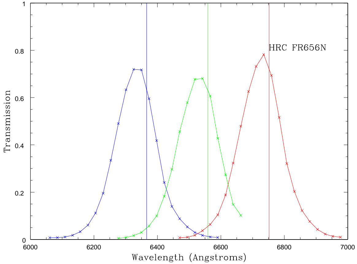
Fig. 1.— Plots of the measured transmission of the ramp filter FR656N on the HRC, set at three central wavelengths: 6366, 6559 and 6752 Å. These wavelengths are shown by the vertical lines. The long-wavelength end of the spectrum of the second setting, with expected central wavelength 6559 Å, was corrupted by a cosmic-ray, and is not shown. These observations were taken as part of CAL 9671.
