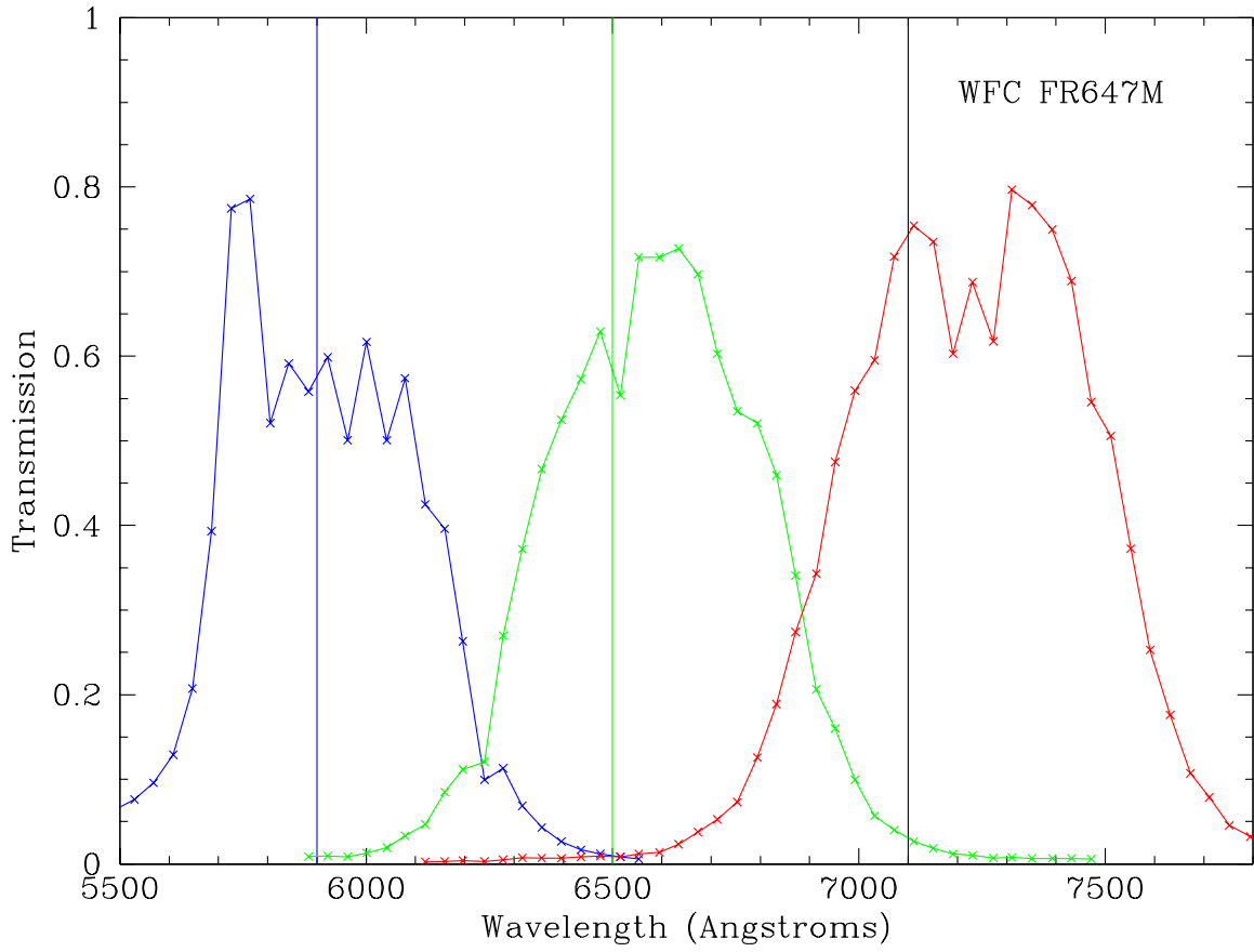
Fig. 7.— Plots of the measured transmission of the ramp filter FR647M on the WFC, set at three central wavelengths: 5900, 6500 and 7100 \text{\AA} , shown by the vertical lines.
