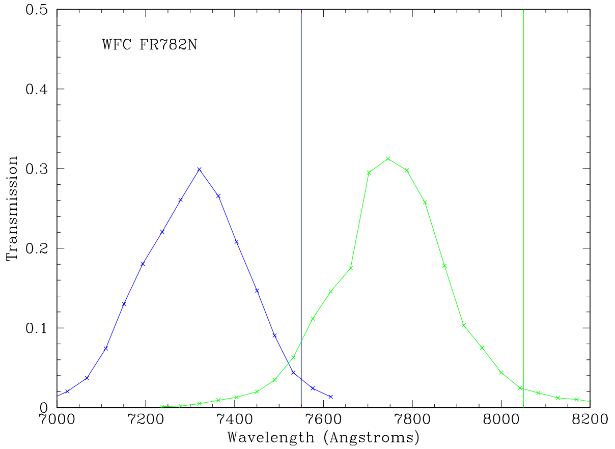
Fig. 9.— Plots of the measured transmission of the ramp filter FR782N on the WFC, set at two central wavelengths: 7550 and 8050 Å.
