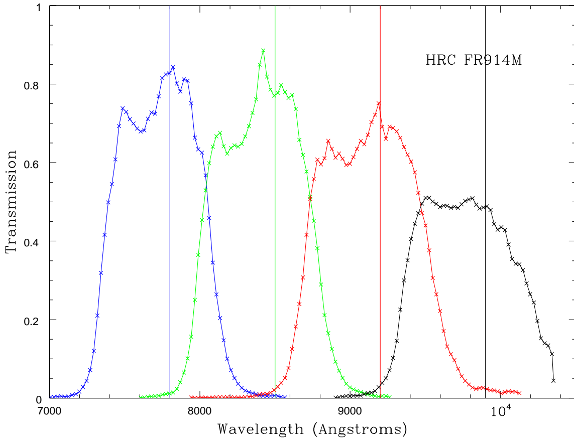
Fig. 4.— Plots of the measured transmission of the ramp filter FR914M on the HRC, set at four central wavelengths: 7800, 8500, 9200 and 9900 Å, shown by the vertical lines. These observations were taken as part of CAL 10742.
