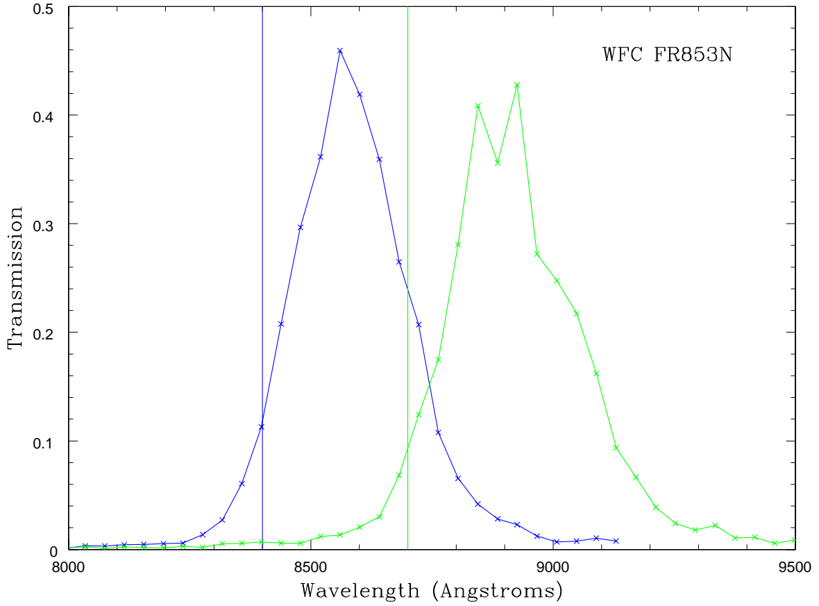
Fig. 8.— Plots of the measured transmission of the ramp filter FR853N on the WFC, set at two central wavelengths: 8400 and 8700 Å.
