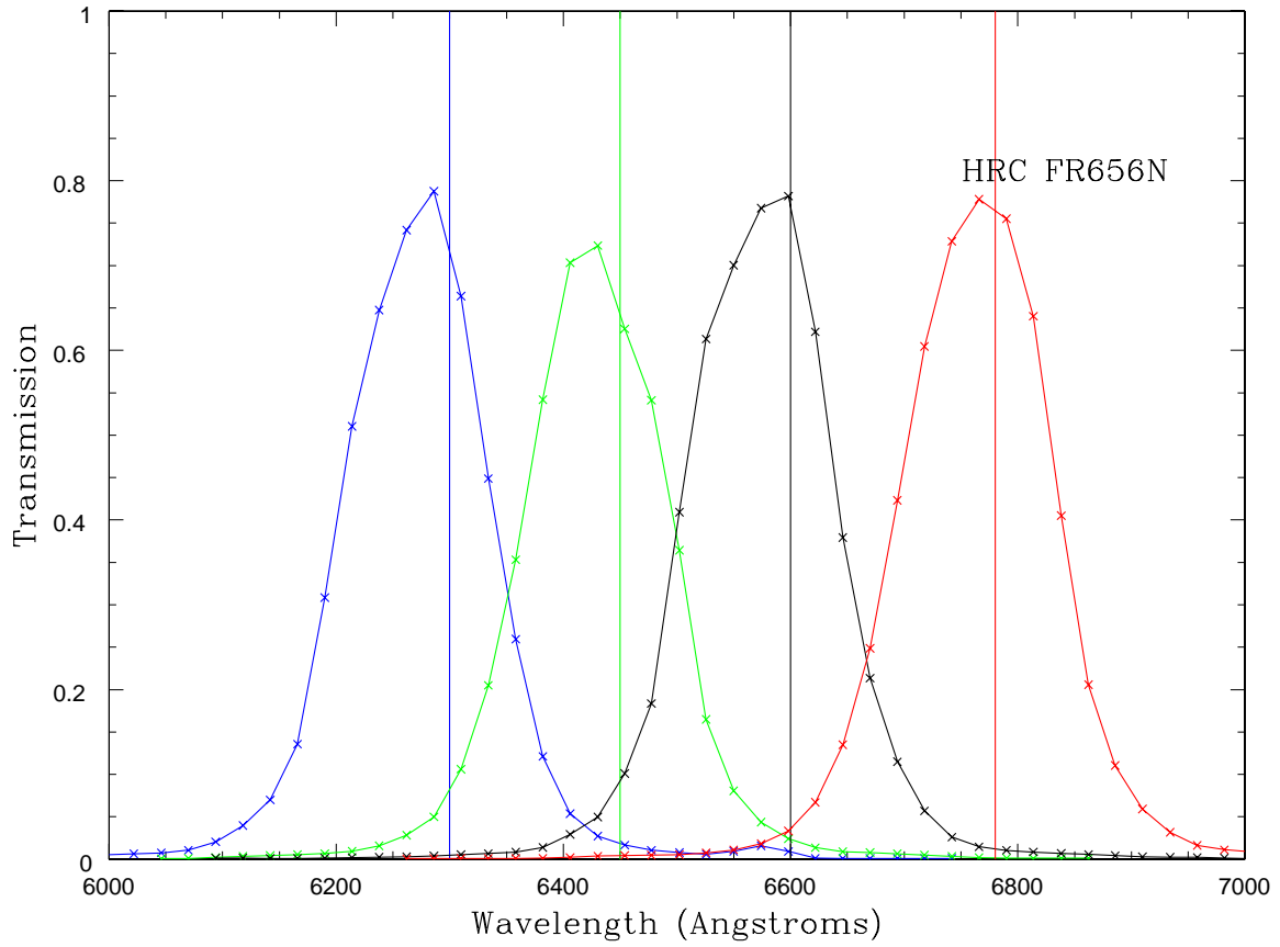
Fig. 3.— Plots of the measured transmission of the ramp filter FR656N on the HRC, set at central wavelengths: 6300, 6450, 6600 and 6780 Å, shown by the vertical lines. These observations were taken as part of CAL 10742.
