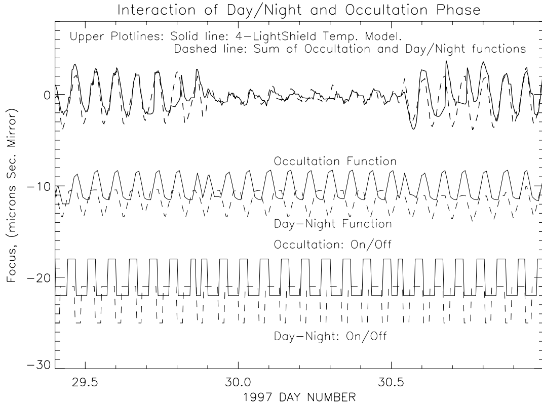
Fig. 2. The effect of day-night and occultation phase on the orbital period temperatures and focus-model amplitudes.
