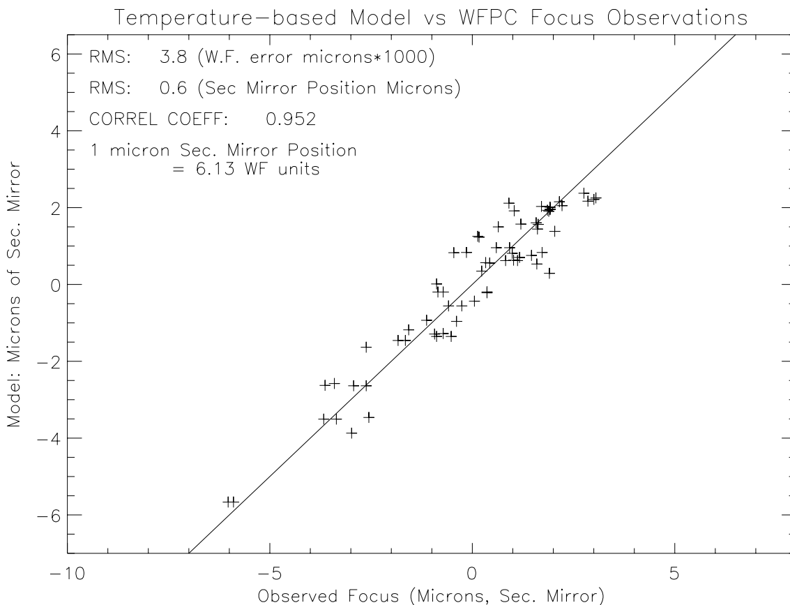
Fig. 6. The correlation of the temperature-based model with the observations of focus for an interval of a month of intensive focus observations in 1997.
