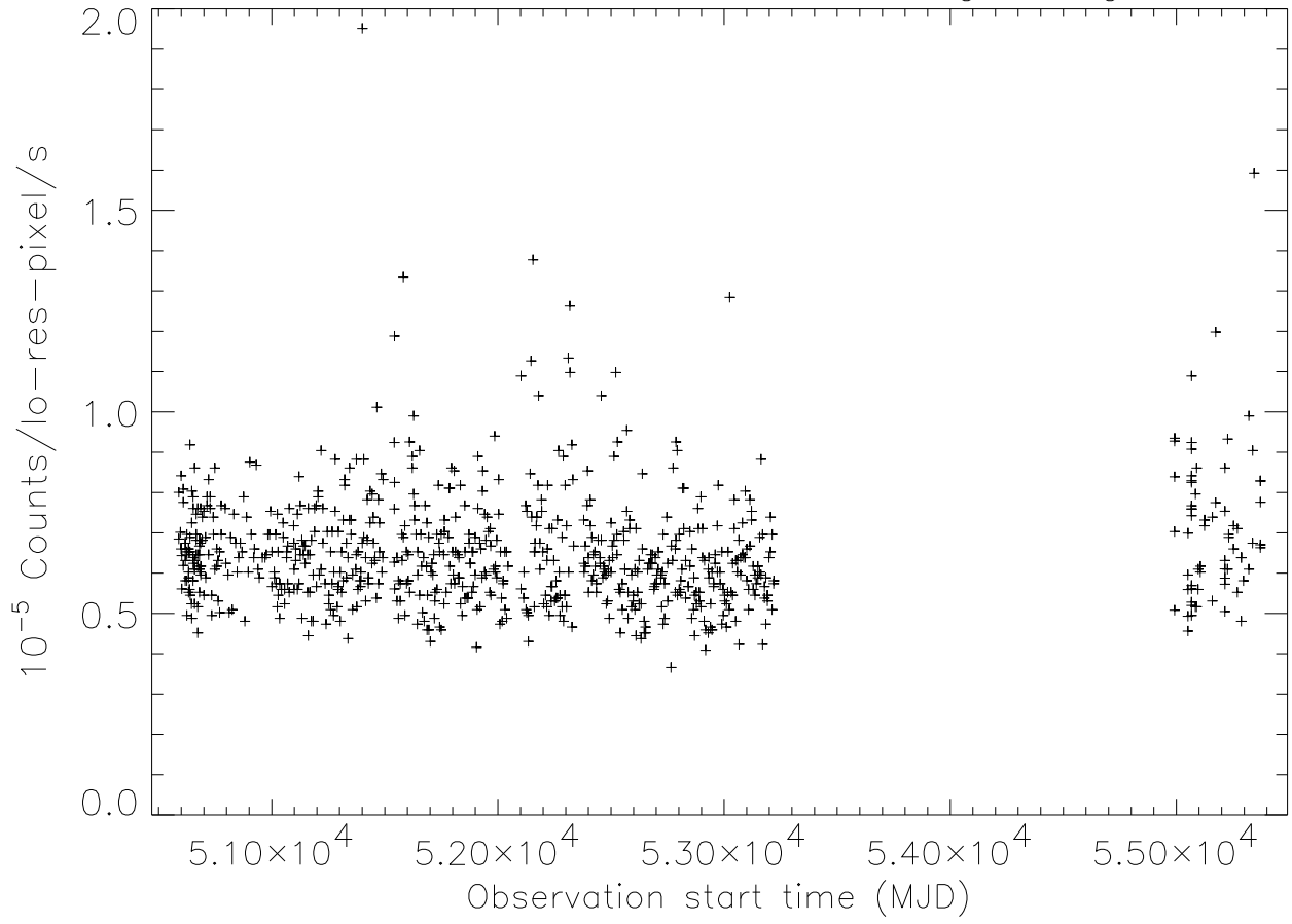
Mean dark rate in FUV MAMA non-glow region
