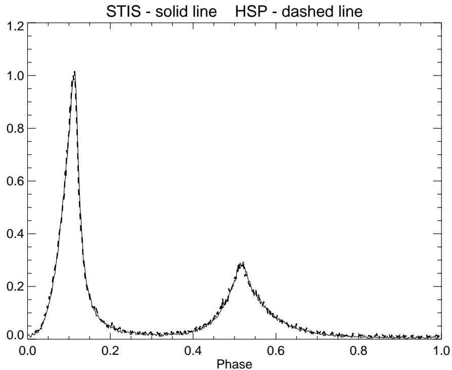
Figure 2. The plot shows the pulse profile constructed from the G230L Crab Pulsar time-tag data (solid line) compared to HSP observations (dashed line) in the same wavelength band (Percival et al., 1993)
