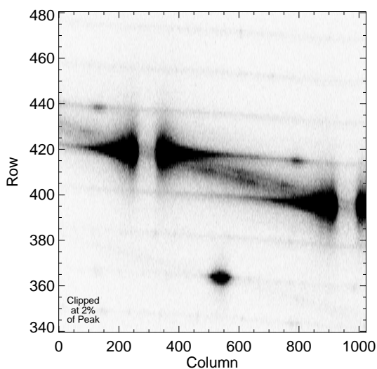
Figure 5: Echelle scatter connects the same double peaked Ly- \alpha emission line in orders 346 (upper) and 347 (lower).
