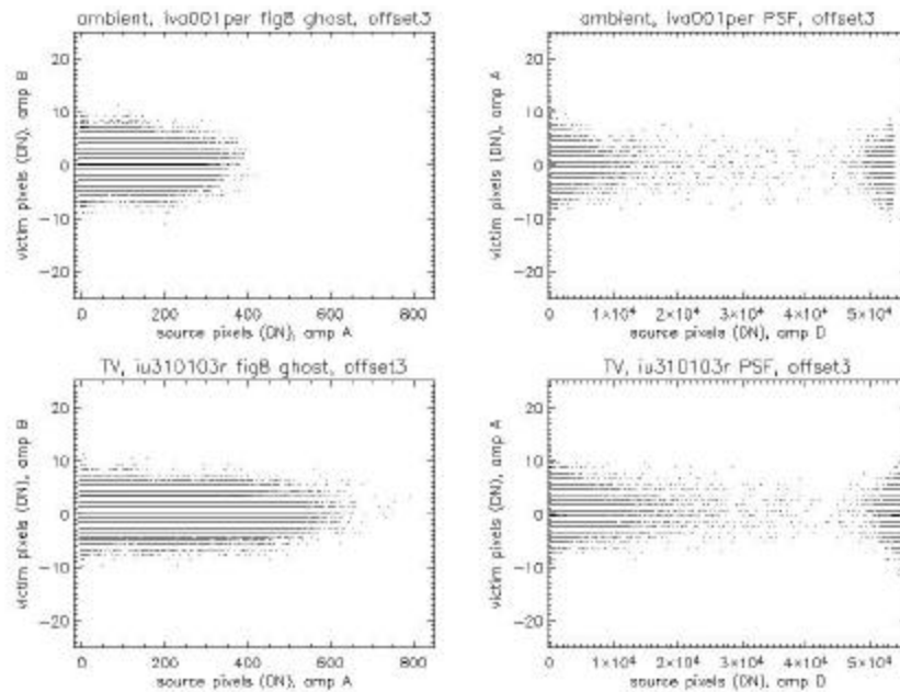
Figure 5: Crosstalk levels in ambient and TV, top and bottom plots respectively. Levels (in DN) in the crosstalk pixels are plotted as a function of source pixel level.
