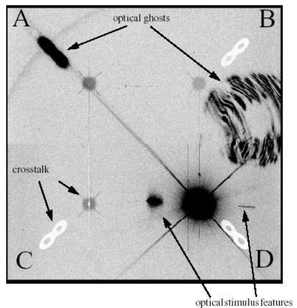
Figure 1: Crosstalk features due to a saturated PSF in quadrant D are visible as circular spots in the center of quads A,B,C. Crosstalk due to the optical ghost in quad A can be seen in quads B,C,D. The image is a gain 1.5, full-frame unbinned four-amp readout obtained during ambient testing, and has been displayed with an extreme hard log inverted stretch in order to highlight the crosstalk features.
