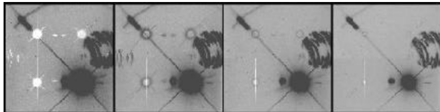
Figure 3: TV crosstalk patterns as a function of gain, with offset level of 3 (gain 1.0, 1.5, 2.0, and 4.0 from left to right).
