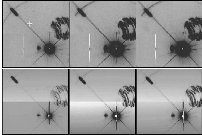
Figure 4: Crosstalk in binned data. Four-amp 2x2 binned and two-amp 3x3 binned images are in the top and bottom rows, respectively. Ambient images are on the left, TV in the middle (bias offset 0) and right (bias offset 3).
