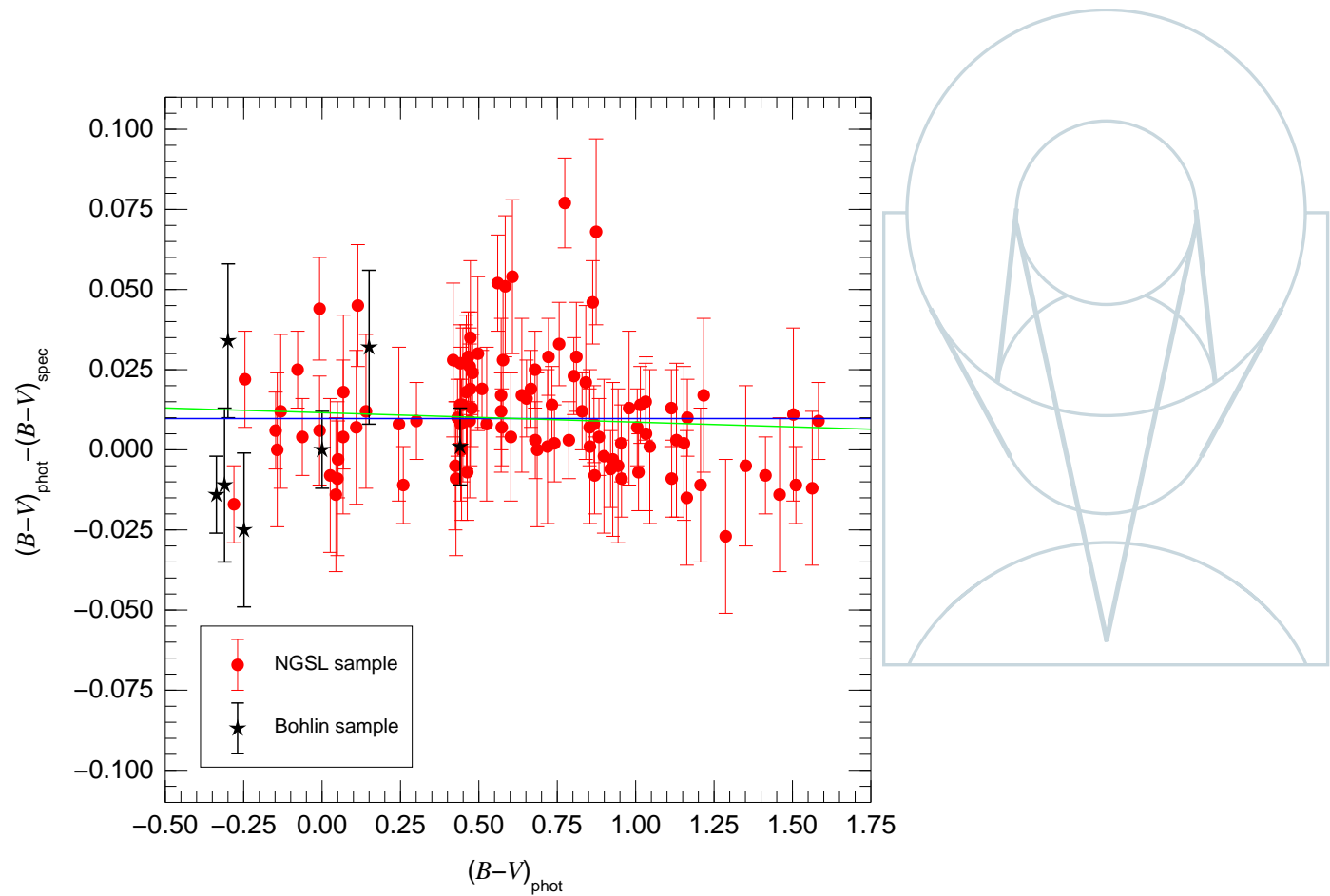
Figure 5. Comparison between photometric and spectrophotometric B - V colors as a function of photometric B - V for the NGSL and Bohlin B - V samples using the Bessell (1990) sensitivity curves. The error bars represent the photometric uncertainties and the horizontal blue line marks the proposed ZP_{B-V} . The green line shows the result of a weighted linear fit to the data.
