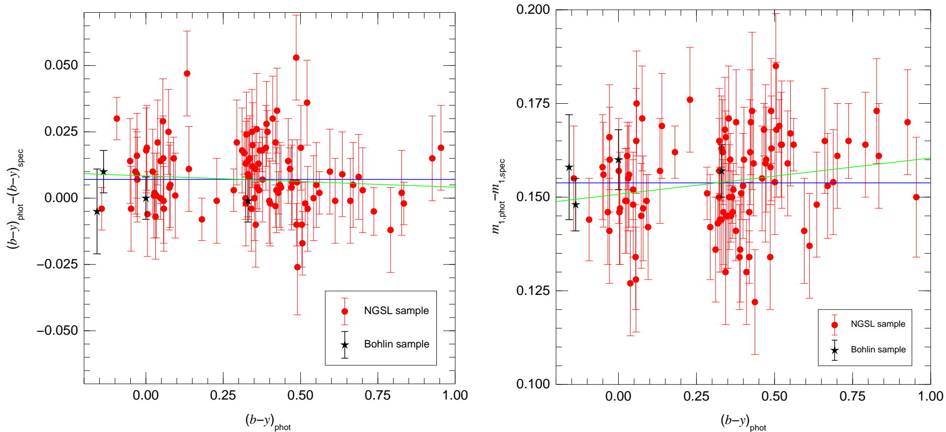
Figure 2. Comparison between photometric and spectrophotometric b - y (left) and m_1 (right) colors as a function of photometric b - y for the NGSL + Bohlin samples using the Matsushima (1969) sensitivity curves. The error bars represent the photometric uncertainties and the horizontal blue line marks the proposed ZP_{b-y} (left) and ZP_{m_1} (right). Green lines show the result of weighted linear fit to the data in each panel.
