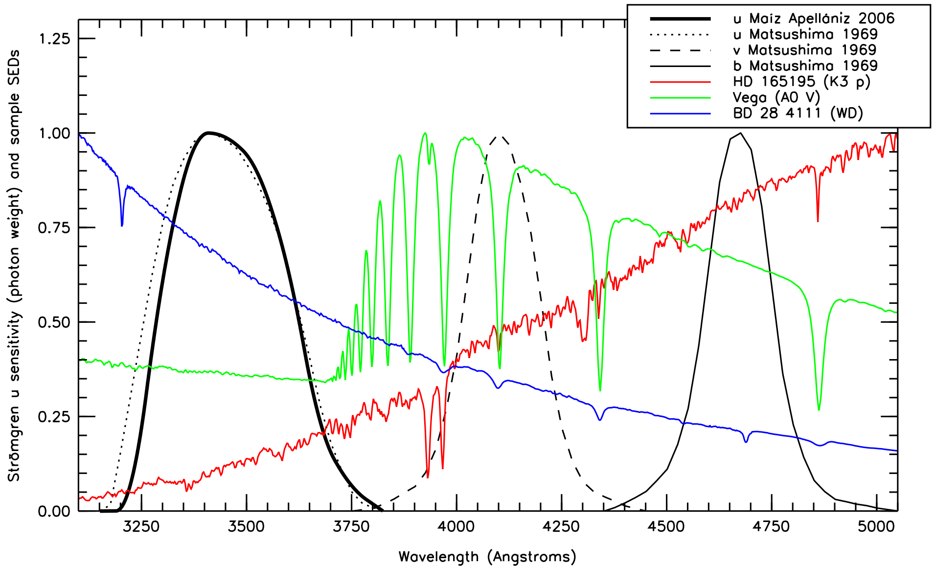
Figure 4. Matsushima (1969) photon-counting normalized sensitivity curves for the the three Strömgen filters u , v , and b filters and the new Maíz Apellániz (2006) curve for u . Three normalized SEDs from the two samples used to calibrate the Strömgen photometry are also shown as f_\lambda .
