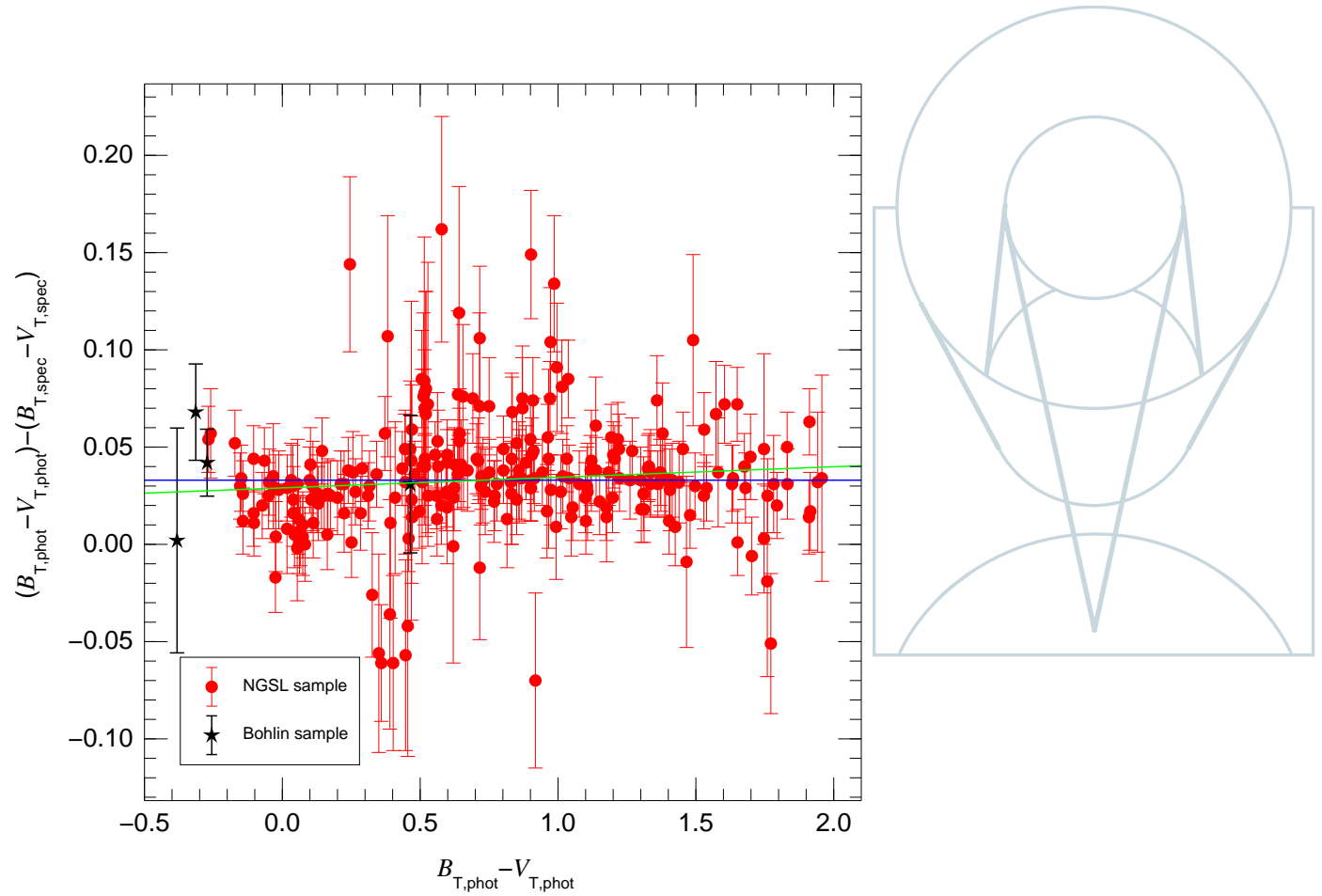
Figure 1. Comparison between photometric and spectrophotometric B_T - V_T colors as a function of photometric B_T - V_T for the NGSL + Bohlin samples using the Bessell (2000) sensitivity curves. The error bars represent the photometric uncertainties and the horizontal blue line marks the proposed ZP_{B_T - V_T} . The green line shows the result of a weighted linear fit to the data.
