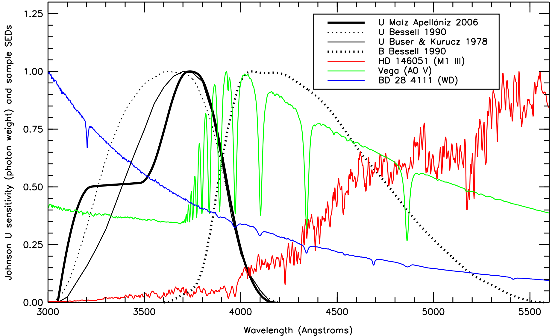
Figure 7. Bessell (1990) U (UX) and B (B) and Buser and Kurucz (1978) U ( U_3 ) photon-counting normalized sensitivity curves and the new Maíz Apellániz (2006) curve for U . Three normalized SEDs from the two samples used to calibrate the Johnson photometry are also shown as f_\lambda .
