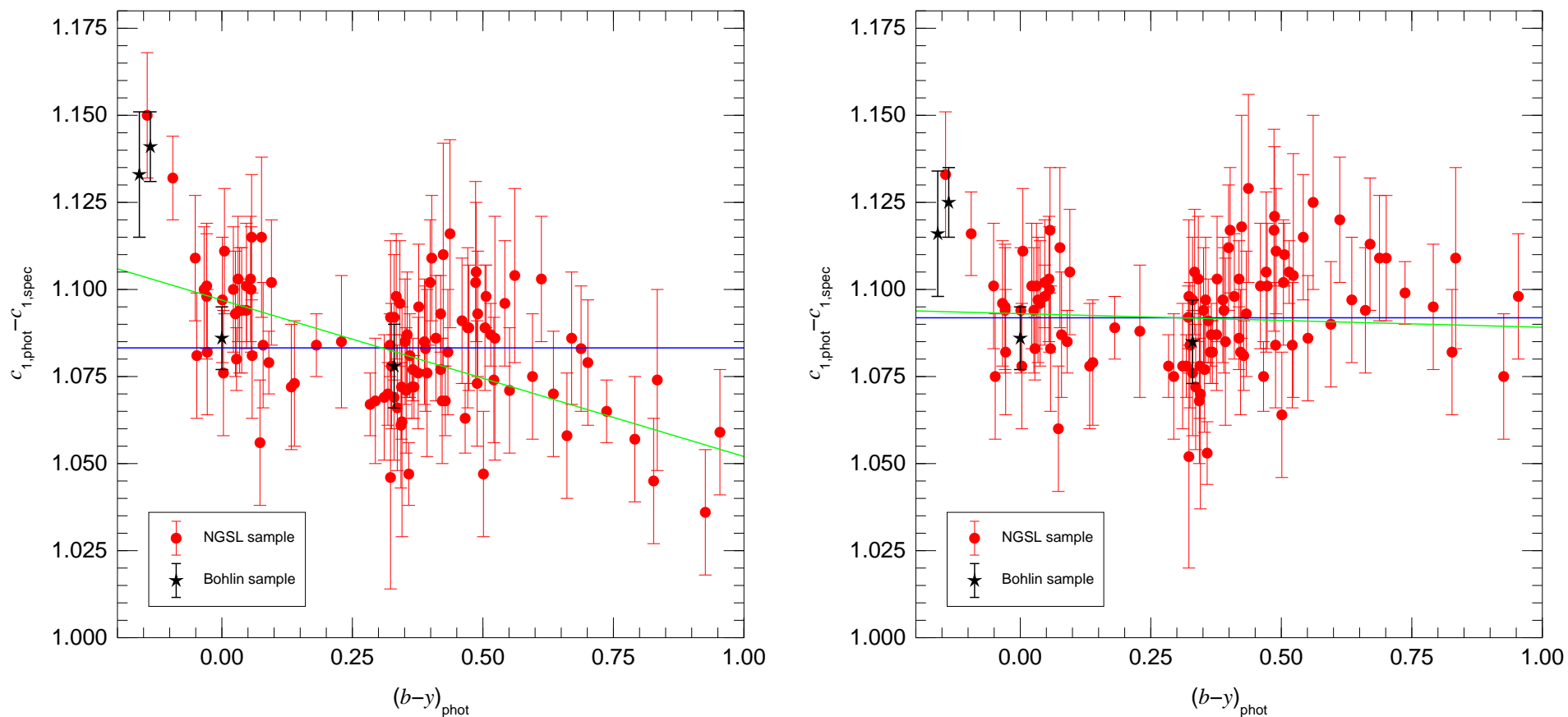
Figure 3. Comparison between photometric and spectrophotometric c_1 indices as a function of photometric b - y for the NGSL + Bohlin samples using the Matsushima (1969) [left] and the Maíz Apellániz (2006) [right] sensitivity curves. The error bars represent the photometric uncertainties and the horizontal blue line marks the weighted mean for the vertical coordinate (which for the right plot represents the proposed ZP_{c_1} ). Green lines show the result of weighted linear fit to the data in each panel.
