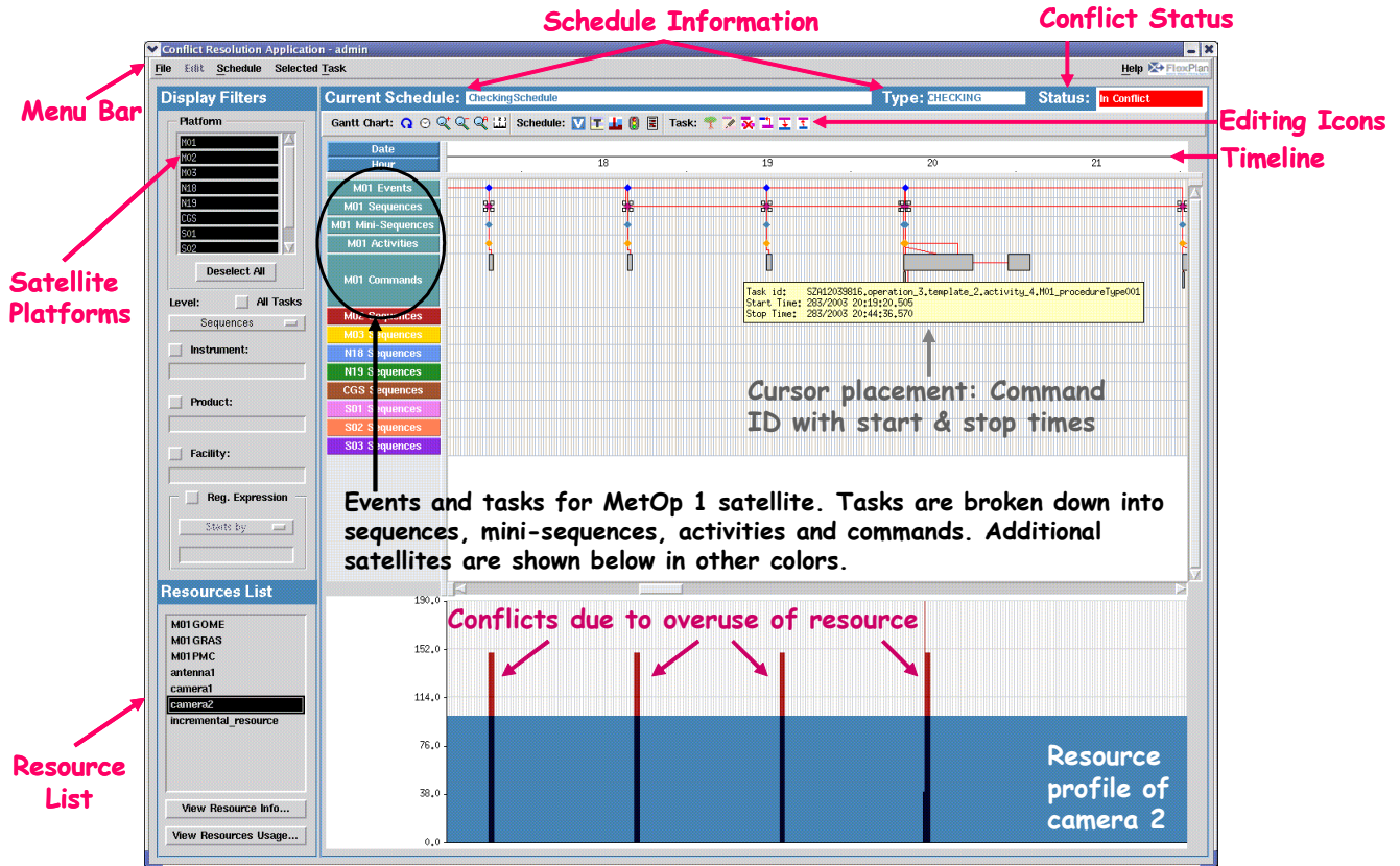
Figure 2: FlexPlan Gantt Chart Screenshot showing Conflicts in the Resource Profile
