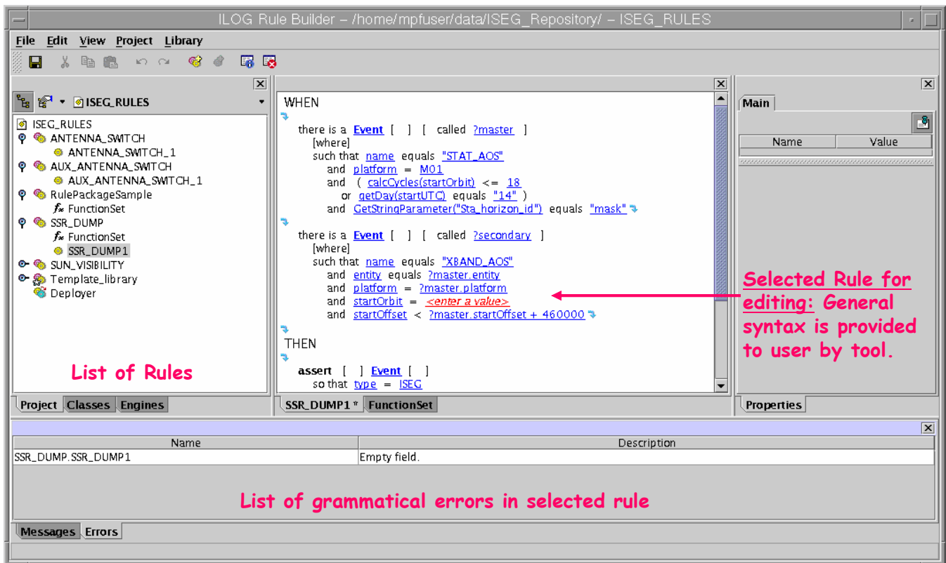
Figure 3: ILOG Rule Builder Screenshot in FlexPlan
