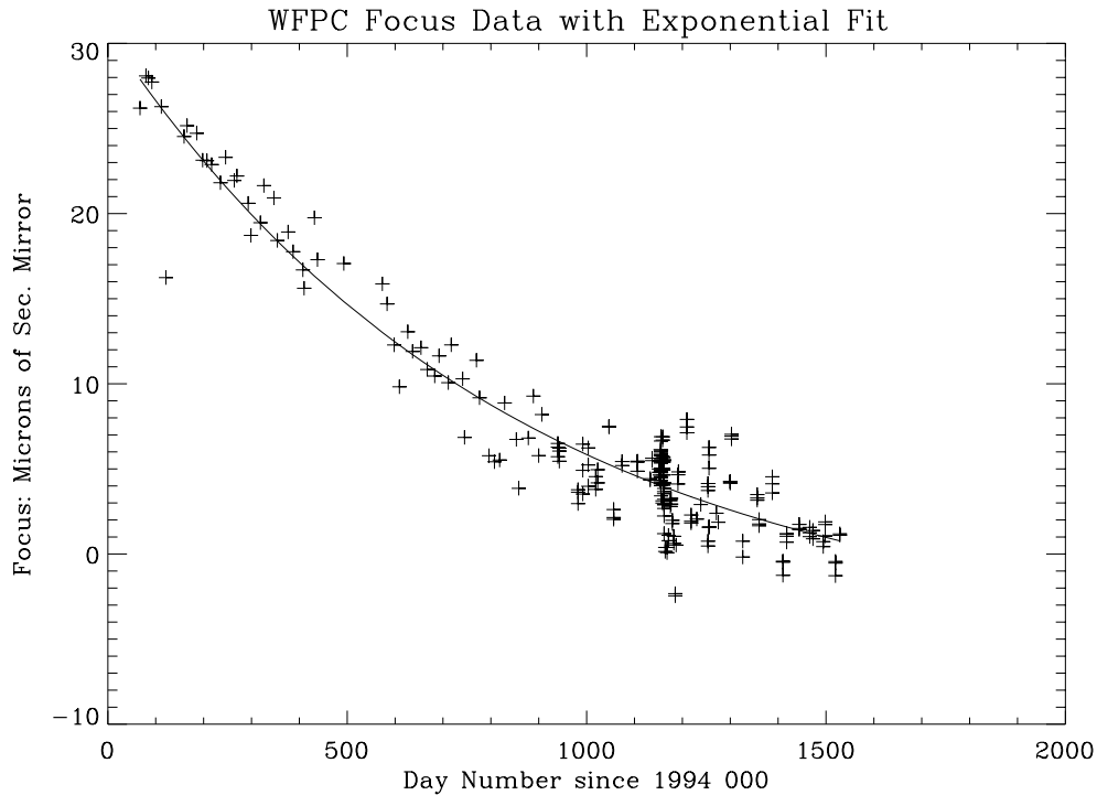
Fig. 8. The focus data since SM1 with the secondary mirror moves restored. The low point at day 121 is a valid observation; it the same observaion shown in Fig. 4b.
