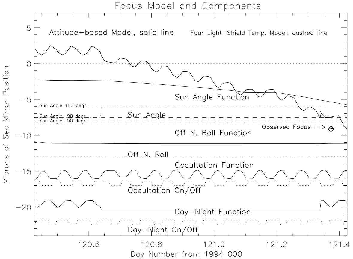
Fig. 4b. A one-day interval showing the case of the largest observed focus deviation, equivalent to -9 microns of secondary mirror motion. No temperatures were available for the 4-temperature based model.
