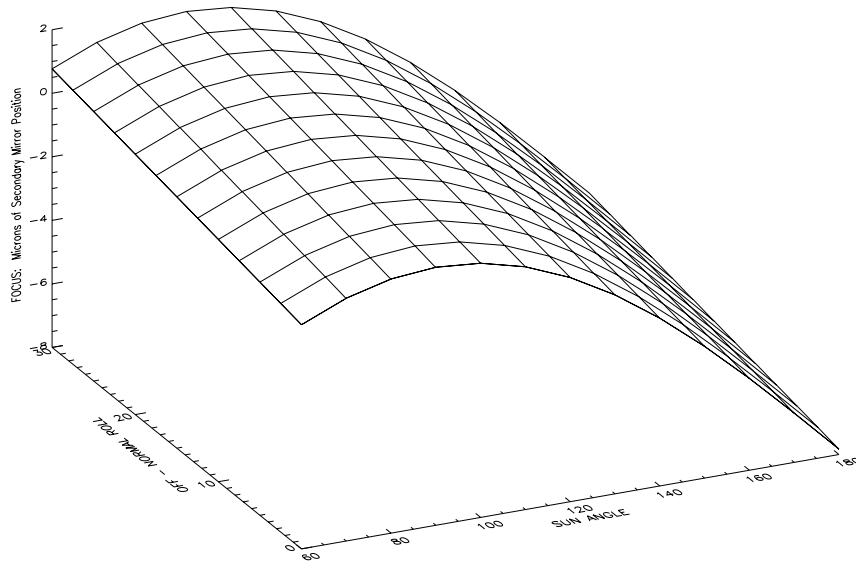
Fig. 10. The dependence of focus on combinations of equilibrium values of only sun-angle and off-normal roll.
