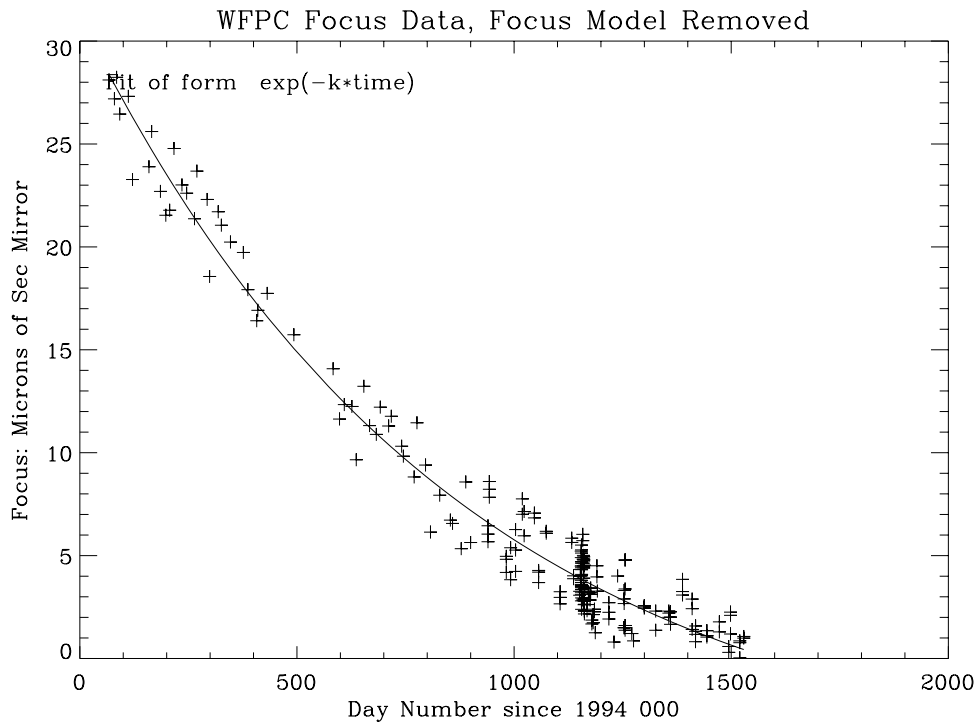
Fig. 9. The focus data with secondary mirror moves restored and the attitude-based focus model removed. The point which fell very low on day 121 in Figs. 7 and 8 has been brought up to the other residuals by the model.
