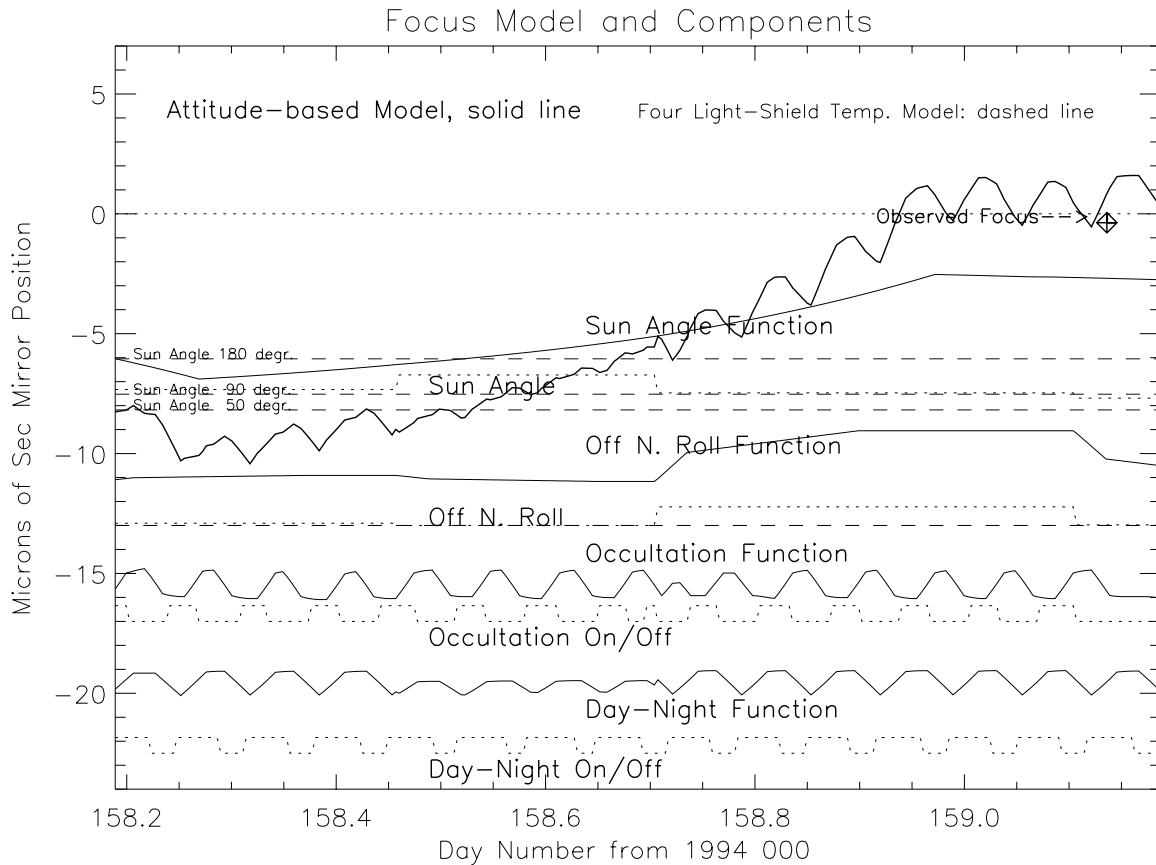
Fig. 4a. A one-day interval showing a case where large sun-angle and off-normal roll changes cause a large excursion in the model, but the model meets the observation at day 159.15. No temperatures were available for the 4-temperature based model.
