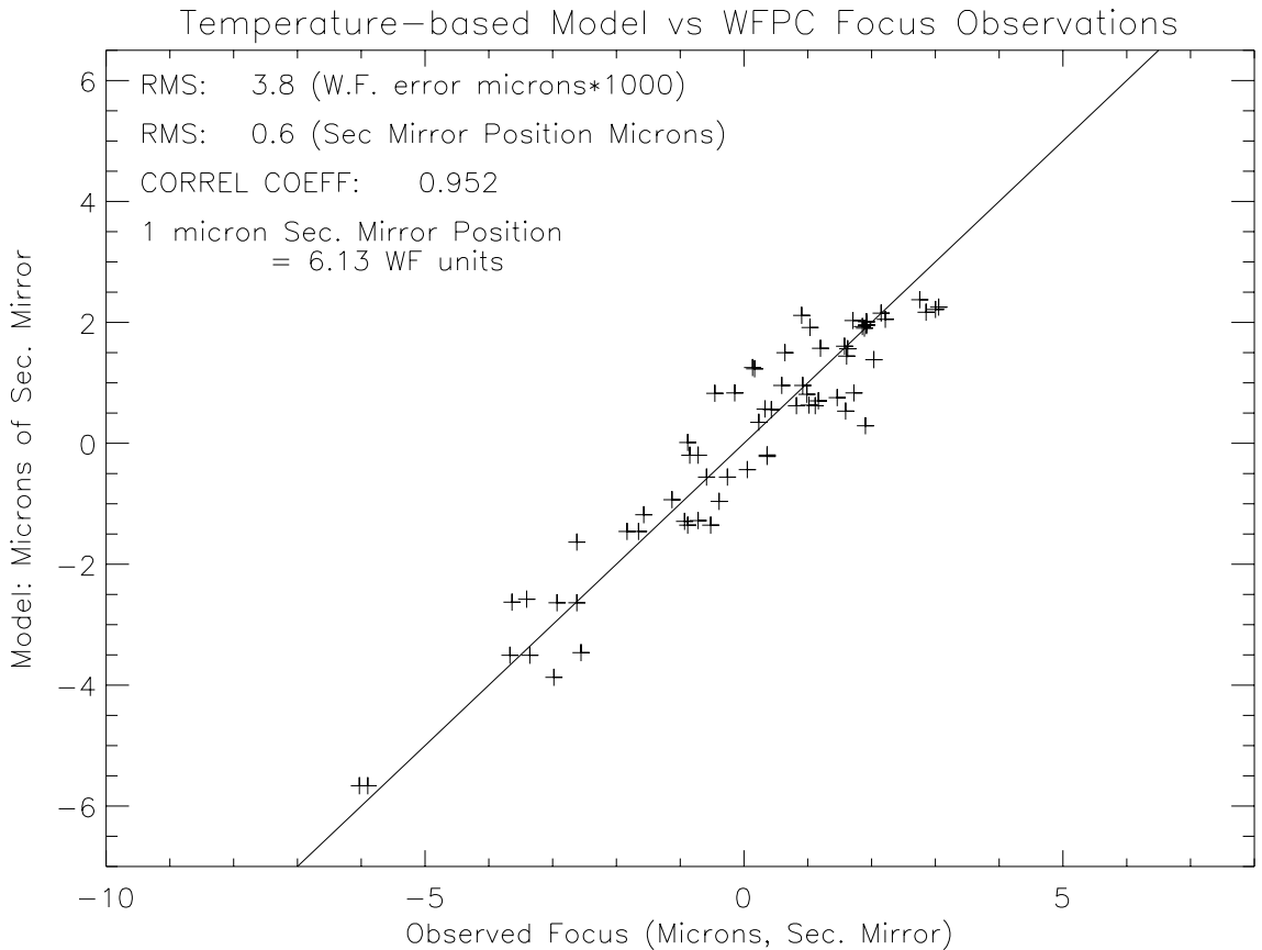
Fig. 6. The correlation of the temperature-based model with the observations of focus for an interval of a month of intensive focus observations in 1997.
