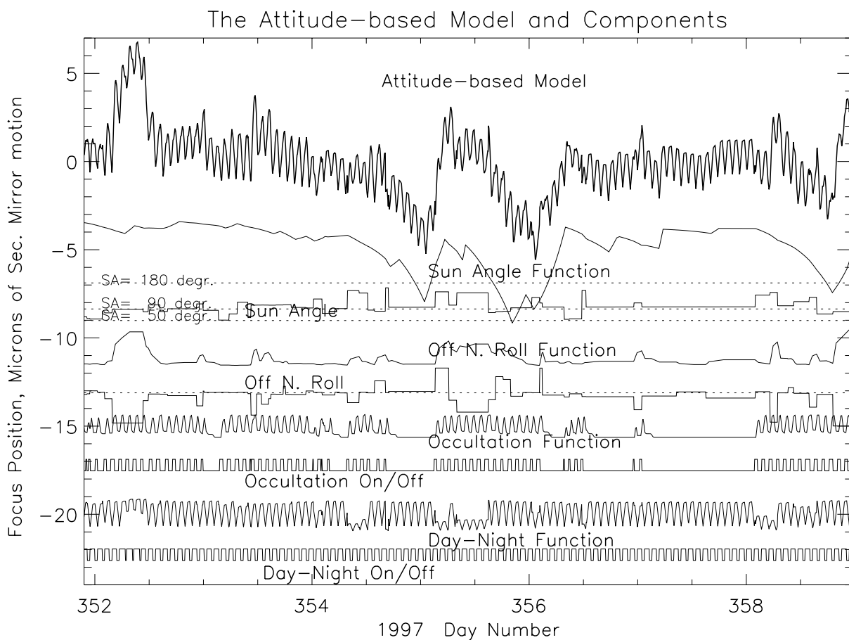
Fig. 3. A week of the attitude-based model and its components.
