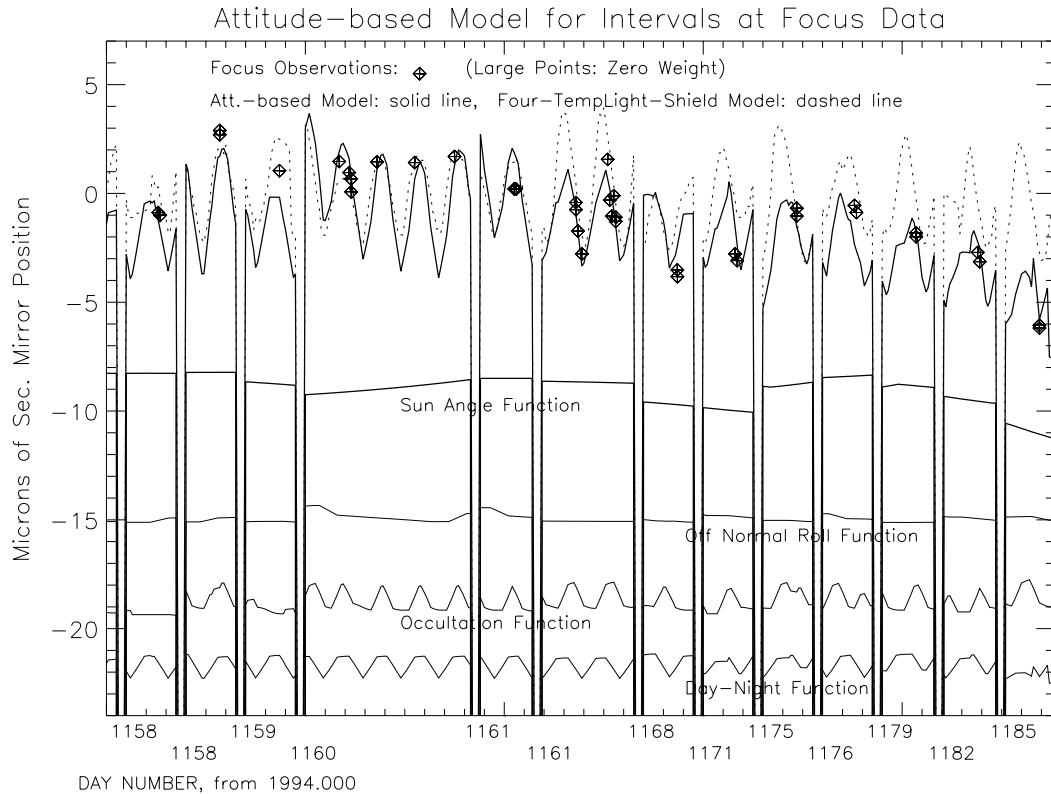
Fig. 5. Focus data and model for a month of relatively intensive focus measurements in 1997. The attitude-based model reaches the rather large downward focus excursion at -6.0 microns on day 1185.
