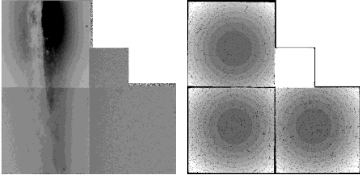
Figure 1. (left) MultiDrizzle output science image, final_sci.fits , with inverted color scale. (right) MultiDrizzle output weight image, final_wht.fits . The display of the weight image has been stretched to highlight the geometric distortion corrections in the WF chips. The gradient from the centers to the edges of the chips is about 3% of the modal WF pixel value. The PC shows a similar effect, but at a level that is outside the image stretch as a result of the difference in the pixel scales of the PC and WF chips.
