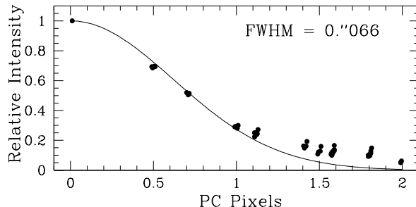
Figure 3. Radial profile of the PSF in the central region of the WFPC2 PC image of Omega Cen taken after SM3B. A composite stellar image was created using about 30 isolated, unsaturated stars near the chip center with the IRAF task psf , and the radial profile measured using the task radprof . The solid line shows the best-fit Gaussian model with \text{FWHM}=0.''066 , comparing well with the pre-SM3B value of 0.''064 .
