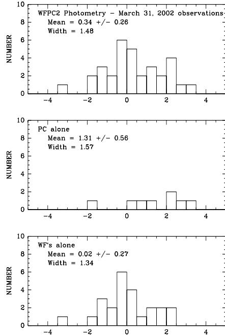
Figure 2. Statistical distribution of the post-SM3B photometry data points around the predicted values based on the fits obtained for each filter independently, and normalized by the 1-sigma error bars for each filter.
