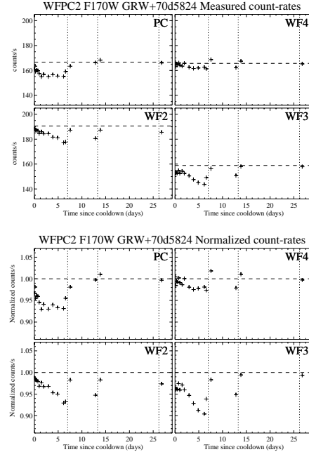
Figure 1. Measured decrease in the observed count-rate of GRW+70d5824 during the first month after cooldown, plotted for each of the cameras separately. The top panels show the measured count-rates, while the bottom panels show count-rates normalized to the pre-SMOV3B values. It can be seen that after each decon, the throughput is effectively returned to its nominal value.
