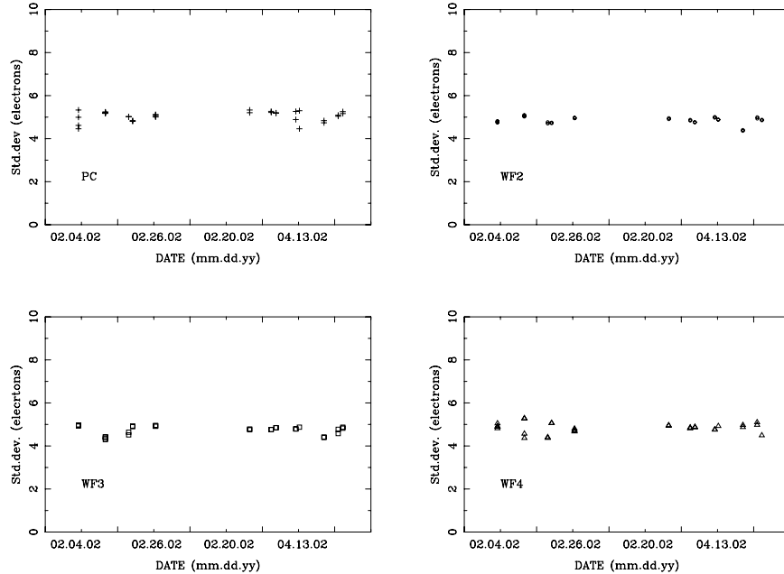
Figure 4. Comparison of the r.m.s. read-noise measured from bias frames taken before and after SM3B, for the four WFPC2 chips (PC, WF2, WF3, WF4), at gain=7. There is no significant change at all in the read-noise for any of the chips, at either gain=7 or 15.
