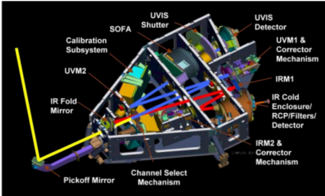
Figure 5. WFC3 Optical Assembly showing UVIS and IR light paths.
