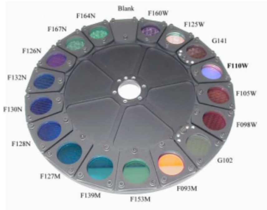
Figure 4. Infrared Filter Wheel.
