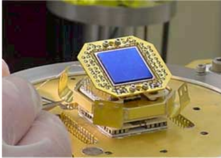
Figure 3. Infrared Focal Plane Array mounted on 6 stage TEC.
