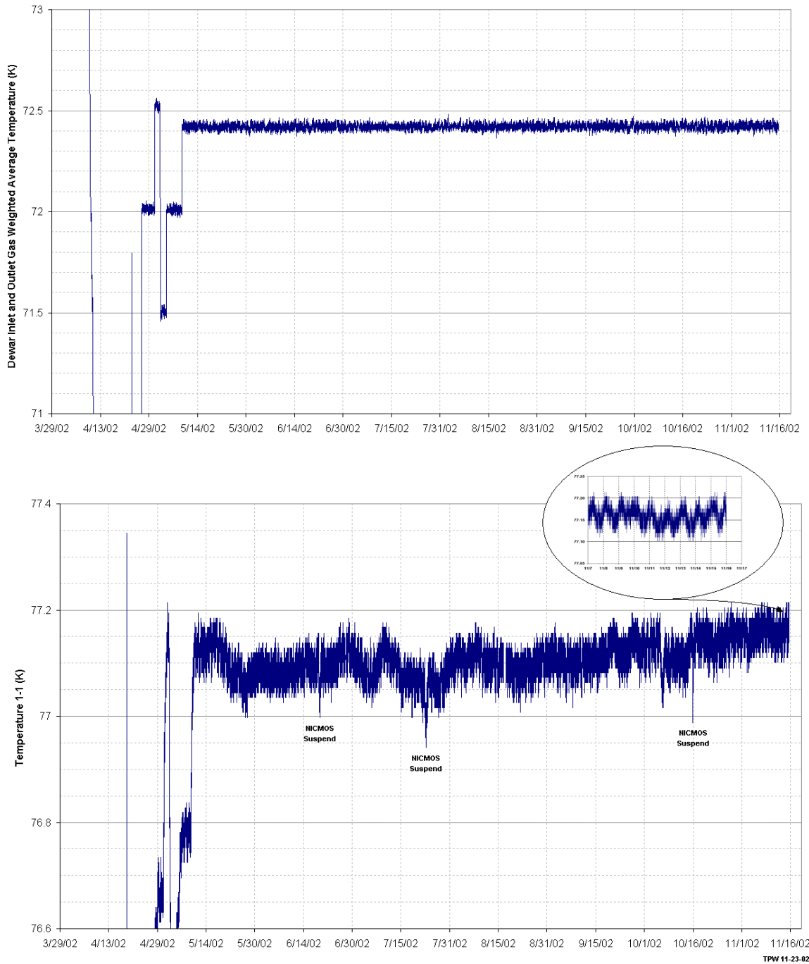
Figure 1. Thermal history of the NCS. Top: weighted average of the Neon inlet and outlet temperature sensors. Bottom: Camera 1 mounting cup sensor which closely traces the actual detector temperature.
