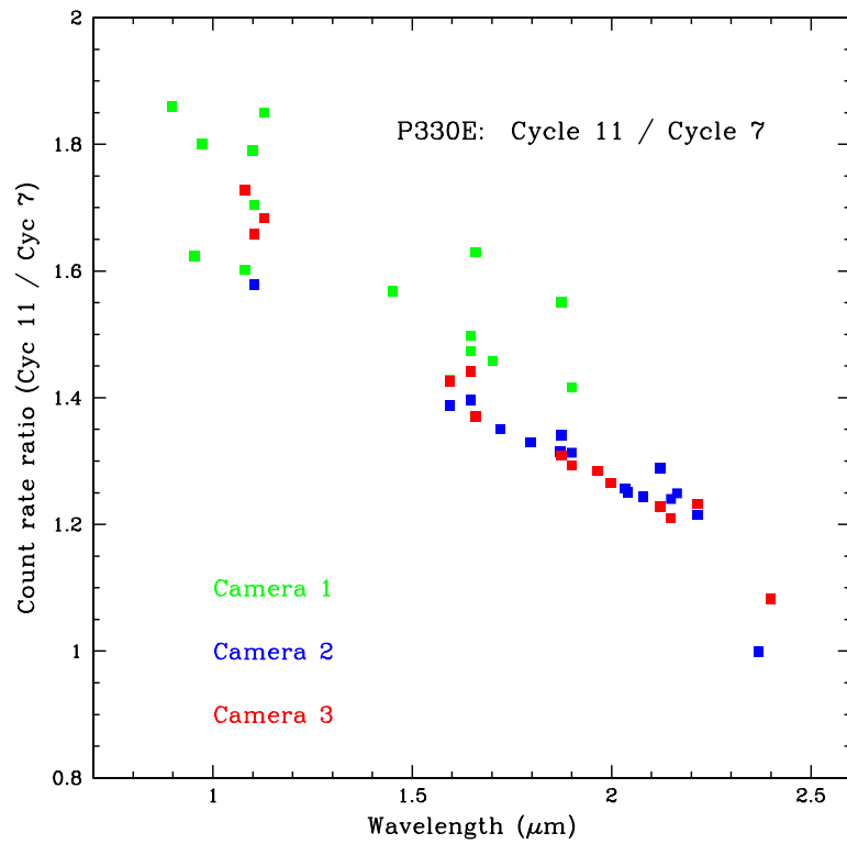
Figure 8. Preliminary comparison of NICMOS sensitivity in Cycle 11 to that from Cycle 7, based on an early analysis of Cycle 11 photometric calibration data for P330E, carried out by Marcia Rieke.
