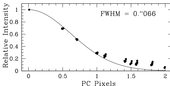
Figure 3. Radial profile of the PSF in the central region of the WFPC2 PC image of Omega Cen taken after SM3B. A composite stellar image was created using about 30 isolated, unsaturated stars near the chip center with the IRAF task psf , and the radial profile measured using the task radprof . The solid line shows the best-fit Gaussian model with \text{FWHM}=0.''066 , comparing well with the pre-SM3B value of 0.''064 .
