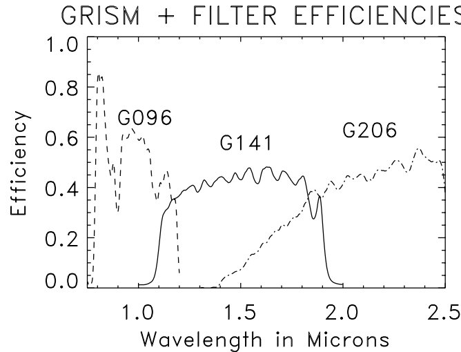
Figure 5. The NICMOS Grism Efficiencies.
