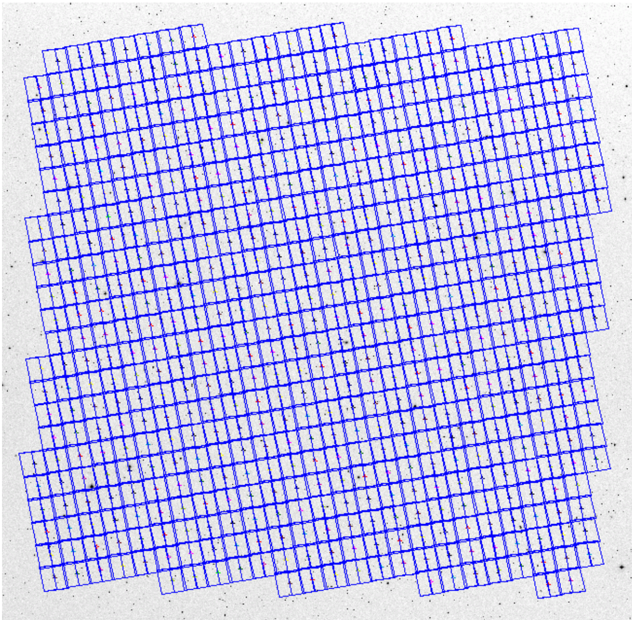
Fig. 1.— The final layout of the full mosaic of all the ACS/WFC F814W pointings, covering a total area of 1.64 \text{ degrees}^2 , or about 77' on a side. The field is centered at 10:00:28.6, +02:12:21.0 (J2000); the rectangle fully enclosing all the ACS imaging has lower left and upper right corners (RA,DEC J2000) at (150.7988^\circ, 1.5676^\circ) and (149.4305^\circ, 2.8937^\circ) .
