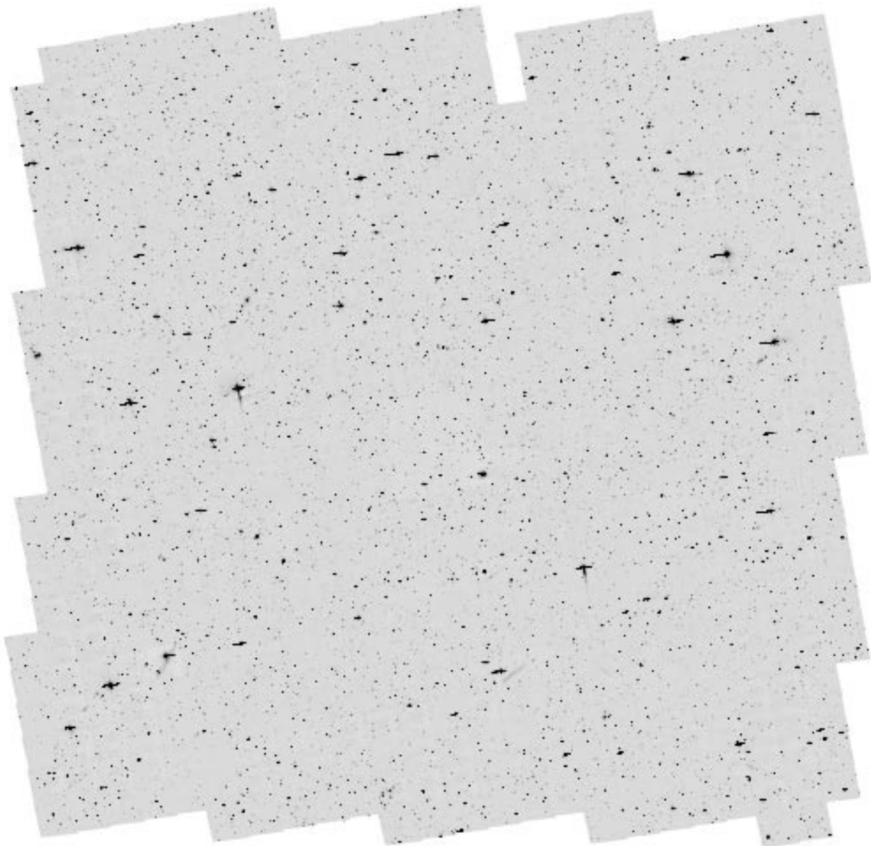
Fig. 4.— The final combined mosaic of all the ACS pointings. At a pixel scale of 0''.05/\text{pixel} , this image has 100800 pixels on a side ( \sim 84' ), with the observations covering an area of 1.64 \text{ degree}^2 . The field is centered at 10:00:28.6, +02:12:21.0 (J2000); the rectangle fully enclosing all the ACS imaging has lower left and upper right corners (RA,DEC J2000) at (150.7988^\circ, 1.5676^\circ) and (149.4305^\circ, 2.8937^\circ) .
