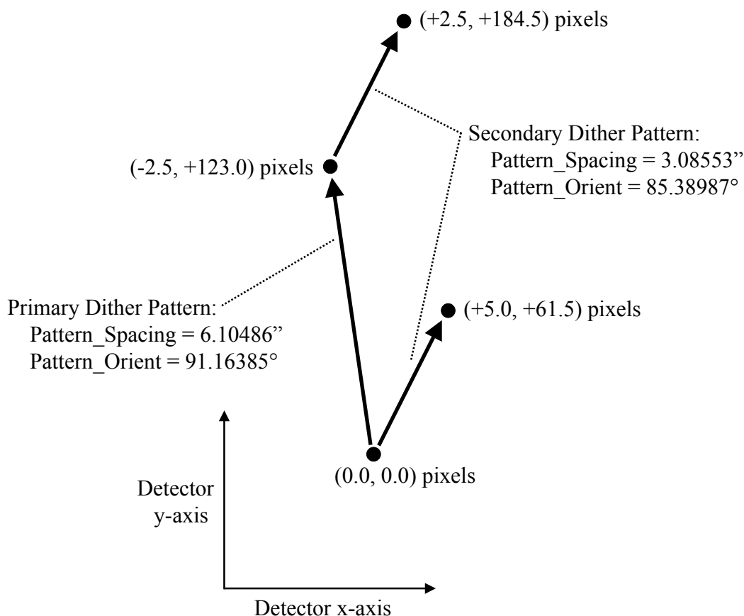
Fig. 2.— Schematic diagram of the dither pattern that we used for each set of four exposures that were obtained for each tile. By combining a 2-point primary dither pattern with a 2-point secondary pattern at each of the two primary dither points, along a slightly different orientation, each of the four pointings was thereby separated in increments of \sim 3'' along the y-axis of the detector and increments of \sim 0''.25 along the x-axis of the detector. The Pattern_Spacing and Pattern_Orient parameters shown are those that were used in the phase II file to construct these offsets. This pattern provided a combination of integer-pixel and half-pixel offsets, thereby ensuring that all four pointings would yield good sampling of any point on the sky by all four quadrants of a detector pixel. The distorted geometry of the detector provides an additional modulation of the phase of this half-pixel subsampling across the image, once all four exposures are combined.
