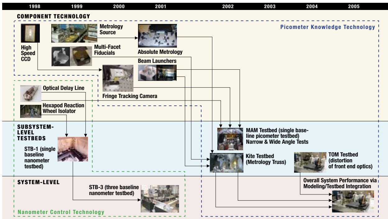
FIGURE 3-1. The SIM Lite technology development program has developed all major technology elements to TRL 6 and therefore to readiness for PDR. Detailed
