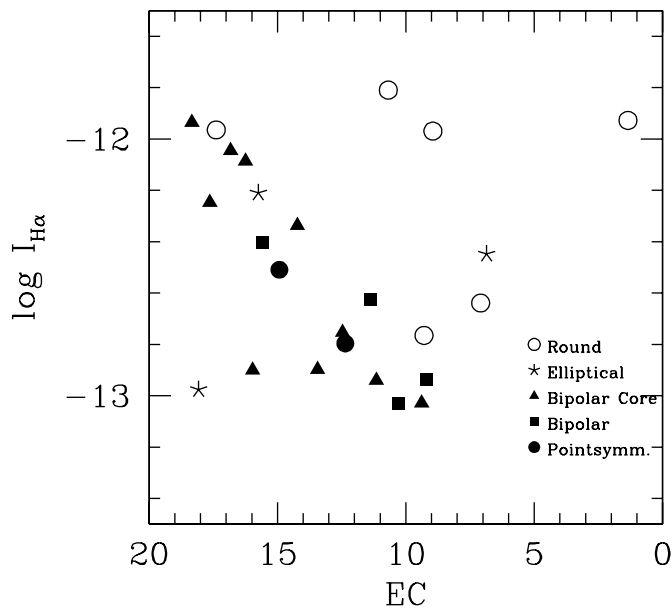
FIG. 11.—Logarithmic H\alpha line intensity vs. excitation constant
