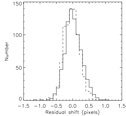
Figure 7. The same as Figure 5 except after a correction to the location of each star using Equation 1 and Table 1 was applied.
