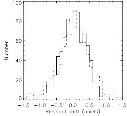
Figure 5. Histogram of the x (solid line) and y (dashed line) residuals after the average shift was subtracted from each pair for the FUV-MAMA.
