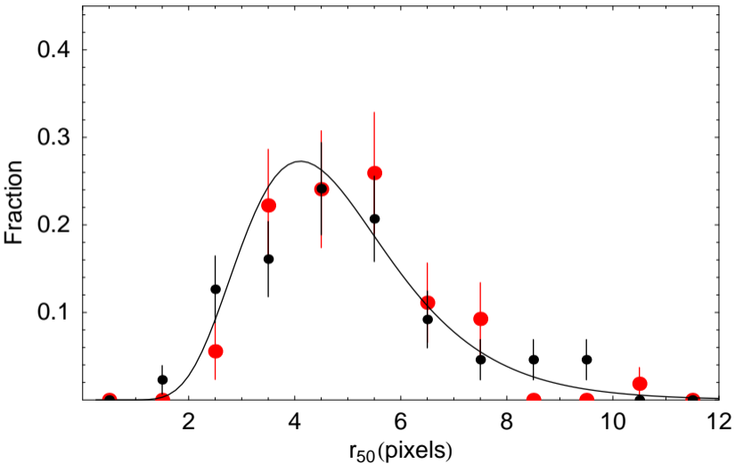
i-dropout r_{50} distribution
