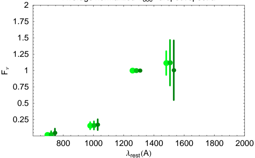
Average normalized V_{606} -dropout spectra
