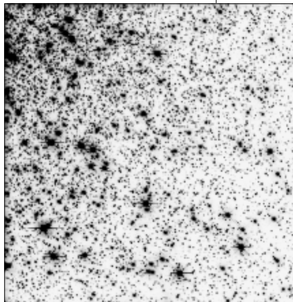
Co-added image for WF3 F555W data. This is the least-crowded of the WFPC2 CCDs, and contains several thousand stars for which time series signal to noise should support planet searches via detection of periodic transit signals of 1 to 6% lasting for 2 to 4 hours.
