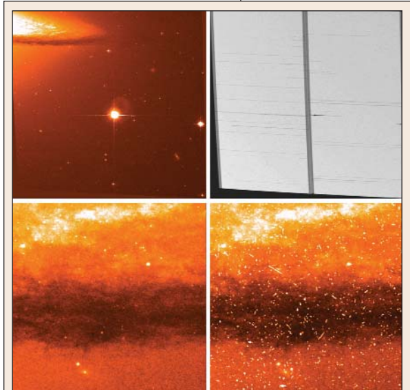
Figure 1: An example of the automatically cleaned MULTIDRIZZLE product, for a four-exposure dithered observation of the nearby galaxy NGC 4594. The top panels show the final, full-frame drizzled and weight images (left and right, respectively). The bottom left panel shows a close-up of the output image from MULTIDRIZZLE, while the bottom right panel shows the same region including all of the accumulated cosmic rays originally present in the exposures.
