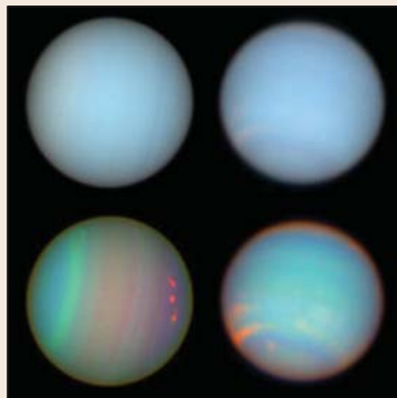
Figure 1: Uranus and Neptune observed by ACS and STIS in a variety of filters. The top panels show the planets in their natural colors, and the bottom panels use an enhanced color representation to highlight atmospheric features. ( http://hubblesite.org/newscenter/newsdesk/archive/releases/2004/05/ )
