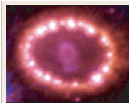
Figure 2: Supernova 1987A was the brightest stellar explosion seen since the one observed by Johannes Kepler 400 years ago. A surrounding ring of gas was in place when the star exploded, probably shed some 20,000 years earlier. This recent Advanced Camera for Surveys image shows many bright spots along the ring of gas, like a 'string of pearls.' They are produced when a supersonic shock wave unleashed during the explosion slams into the gas ring, at more than a million miles per hour.
