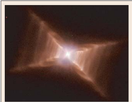
Figure 3: Wide Field and Planetary Camera 2 image of one of the most unusual nebulae known in our Milky Way, HD 44179. The nebula is more commonly called the 'Red Rectangle' because of its unique shape and color as seen with ground-based telescopes. The star in the center of the Red Rectangle began its life as a star similar to the sun, but is now ejecting its outer layers to produce the visible nebula. The X-shaped structure is due to the bi-conical geometry of the outflow. In a few thousand years, when ultraviolet light from the star makes the nebula fluoresce, the object will become a planetary nebula.
