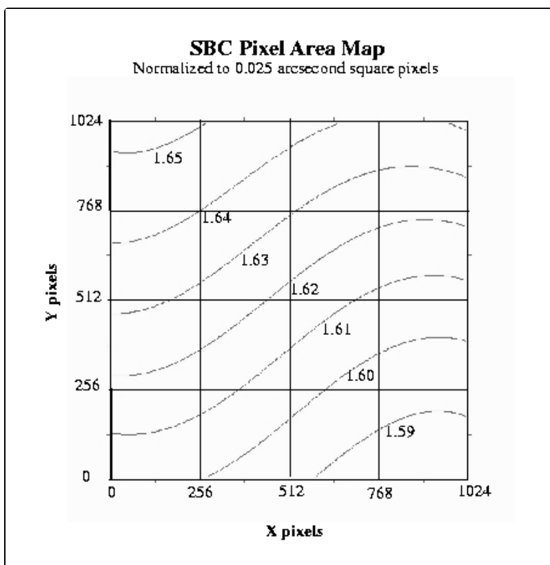
Figure 10.116: The map of the effective pixel areas of the ACS/SBC. The areas are normalized to 0.025 arcsecond square pixels.
