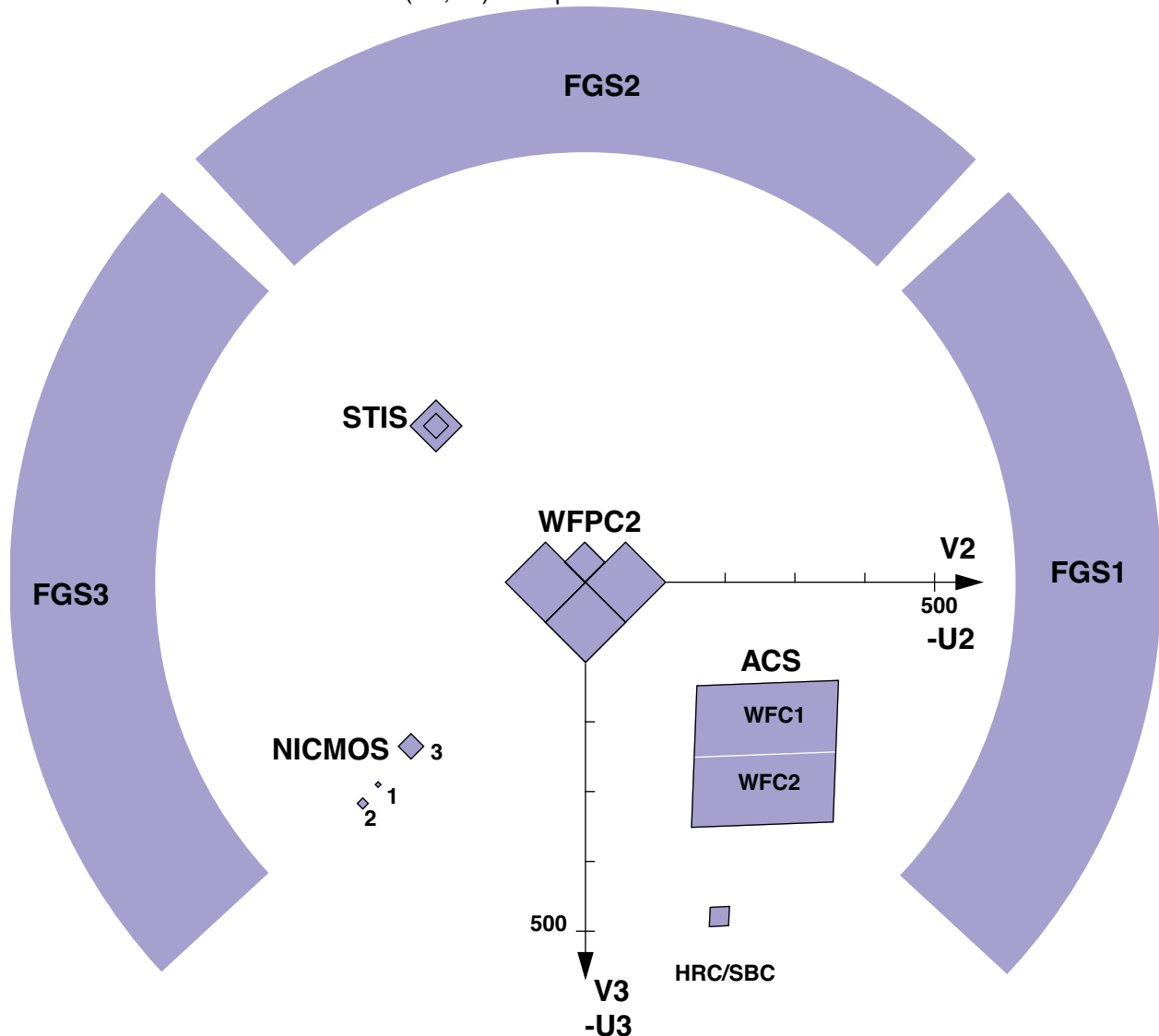
Figure 2.2: The HST field of view with the locations of the SI and the FGS apertures in the (U2,U3) focal plane. The scale in arcsec is indicated.
