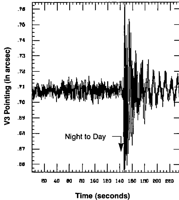
Figure 5.3: FGS2 Guide Star Motion at the Onset of a Day/Night Transition
