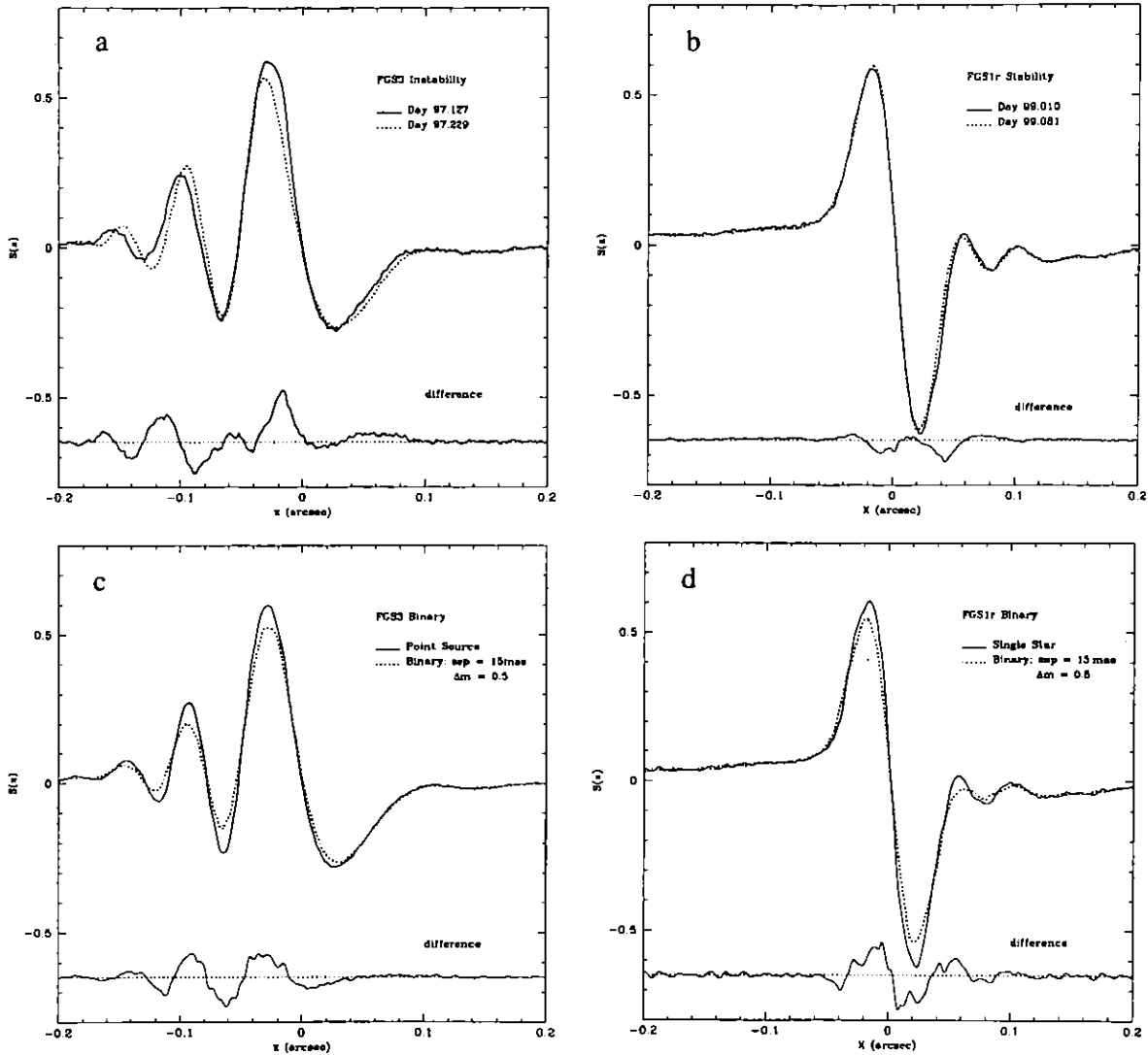
Figure 5.5: Temporal Stability: FGS3 v. FGS1r
