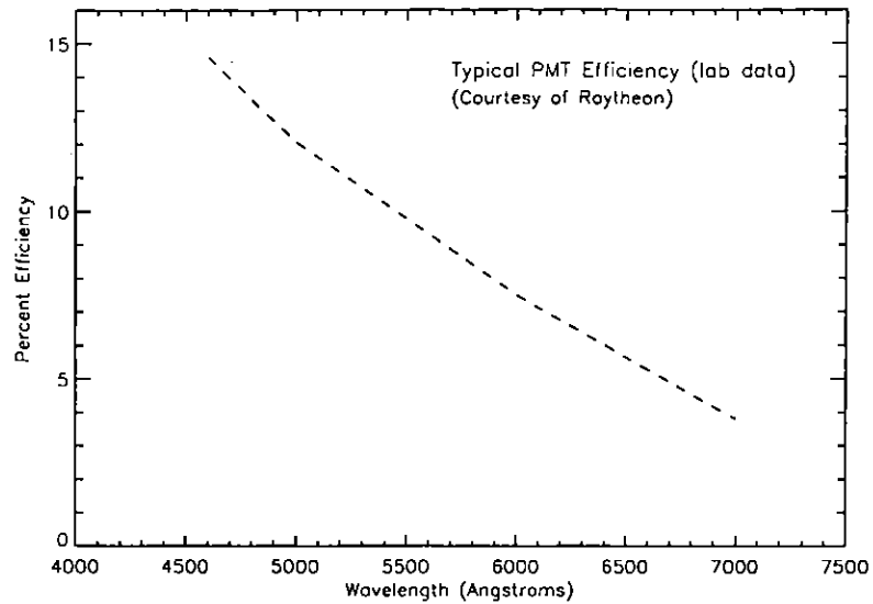
Figure 2.9: PMT Efficiency
