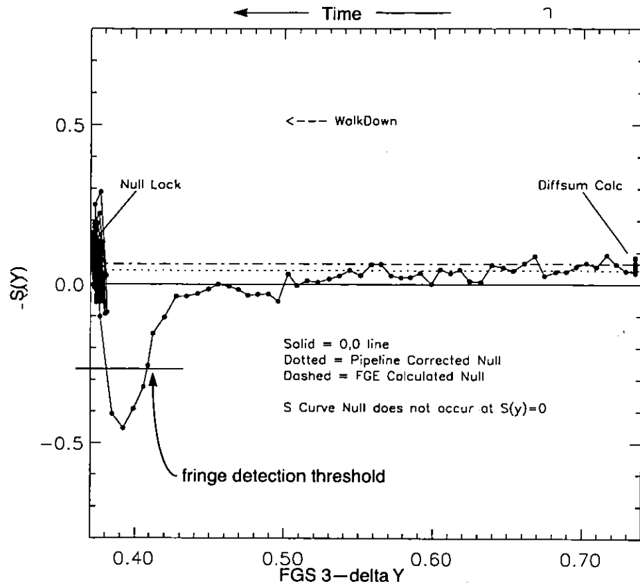
Figure A.2: Offset of True Null from S_y=0
