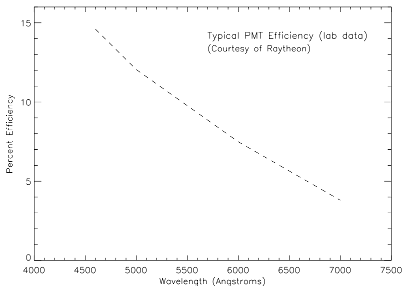
Figure 2.9: PMT Efficiency
