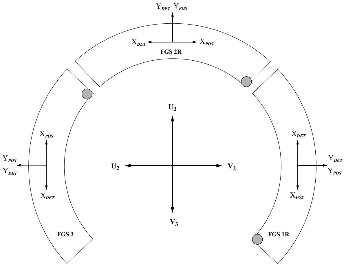
Figure 2.10: FGS Proposal System and Detector Coordinate Frames
