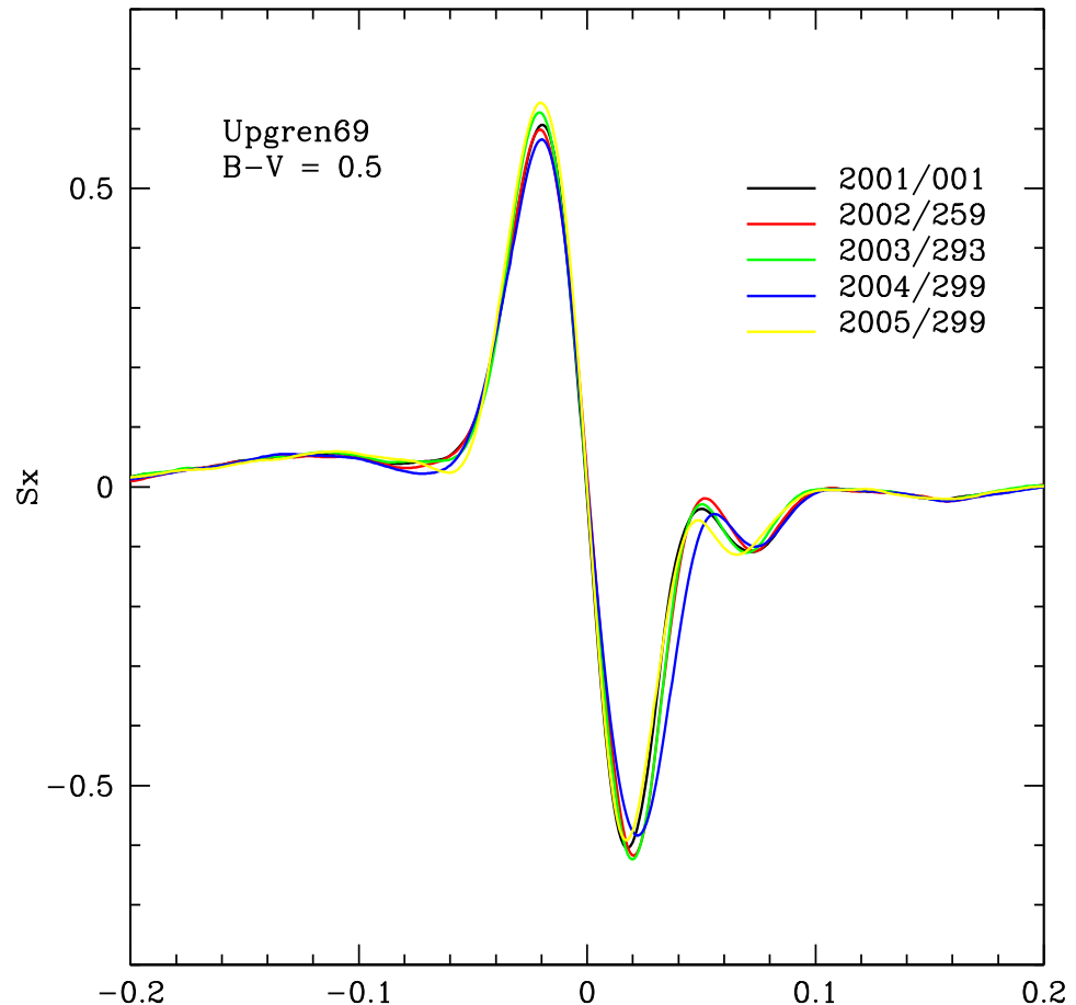
Figure 4.5: Evolution of S-curve morphology along the FGS1r Y-axis
