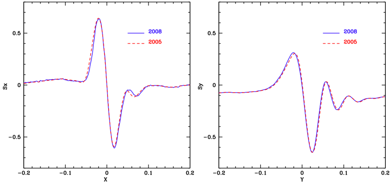
Figure 2.8: FGS1r S-curves 2005
