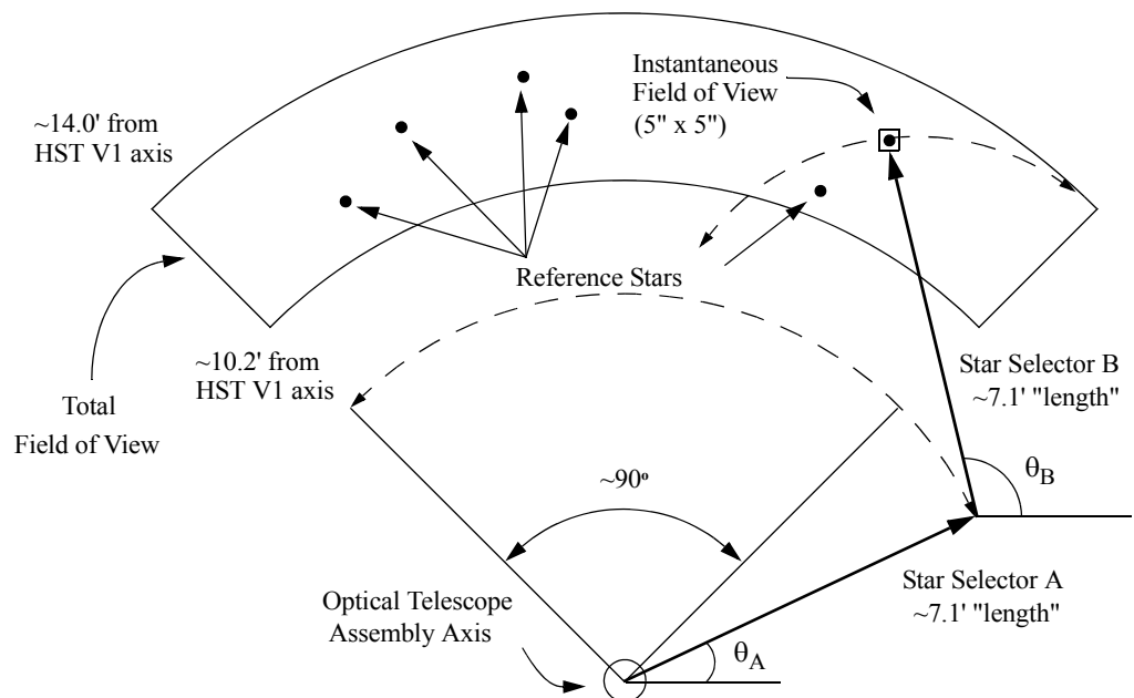
Figure 1.3: FGS Star Selector Geometry
