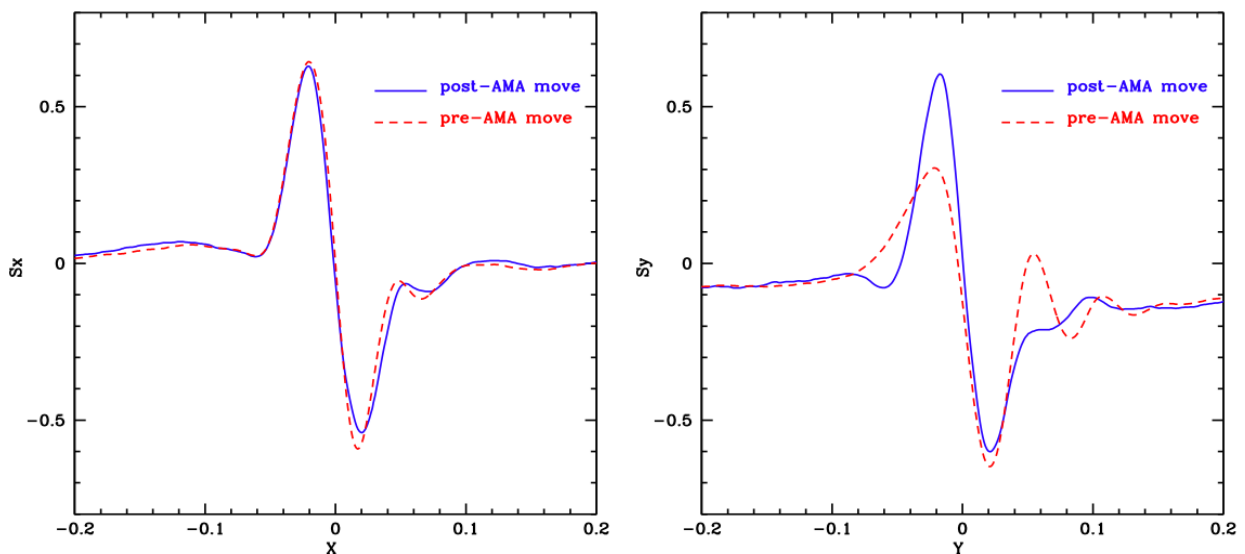
Figure 2.9: Shows the changes in the FGS1r S-curves resulting from the January 2009 AMA adjustment.
