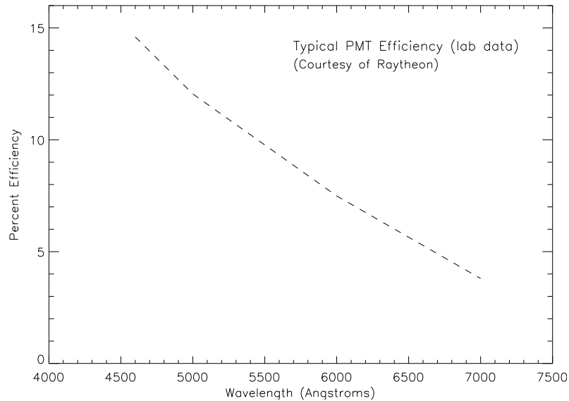
Figure 2.12: PMT Efficiency
