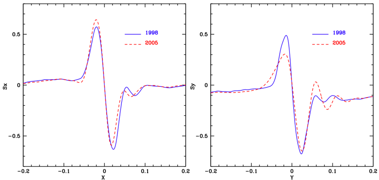
Figure 2.7: FGS1r S-curves
