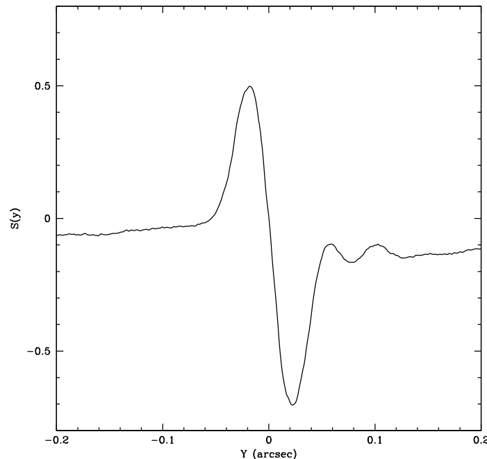
Figure 1.1: FGS Interferometric Response (the “S-Curve”)
