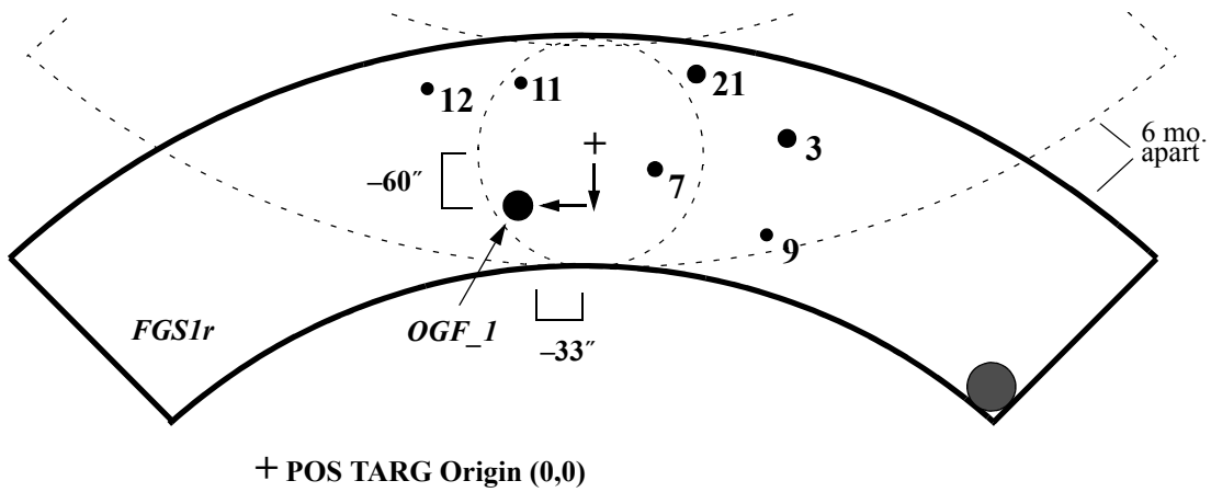
Figure 6.1: Example 1: Field of View at Special Orientation
