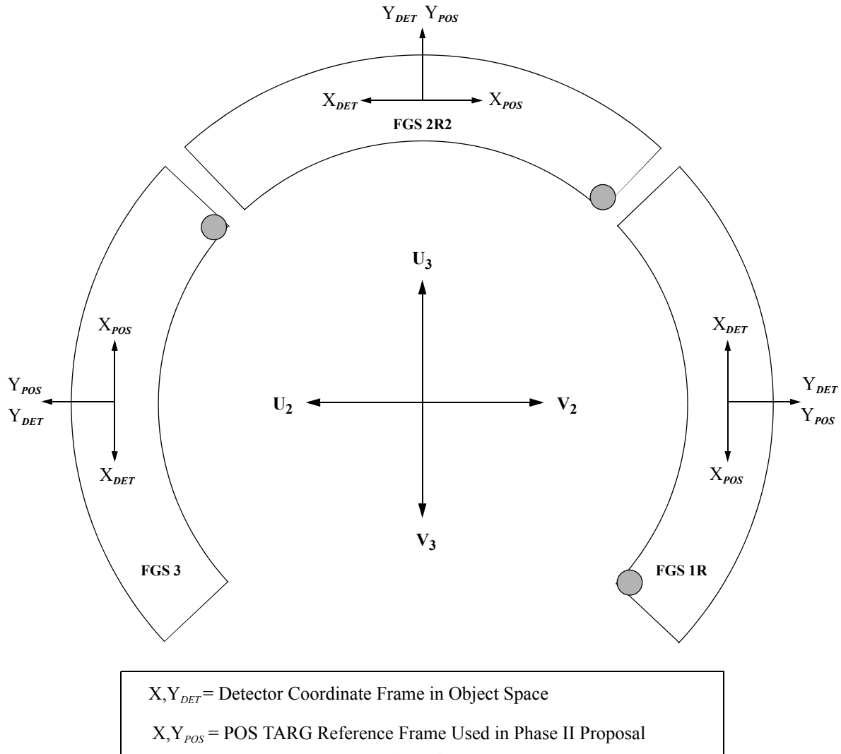
Figure 2.10: FGS Proposal System and Detector Coordinate Frames
