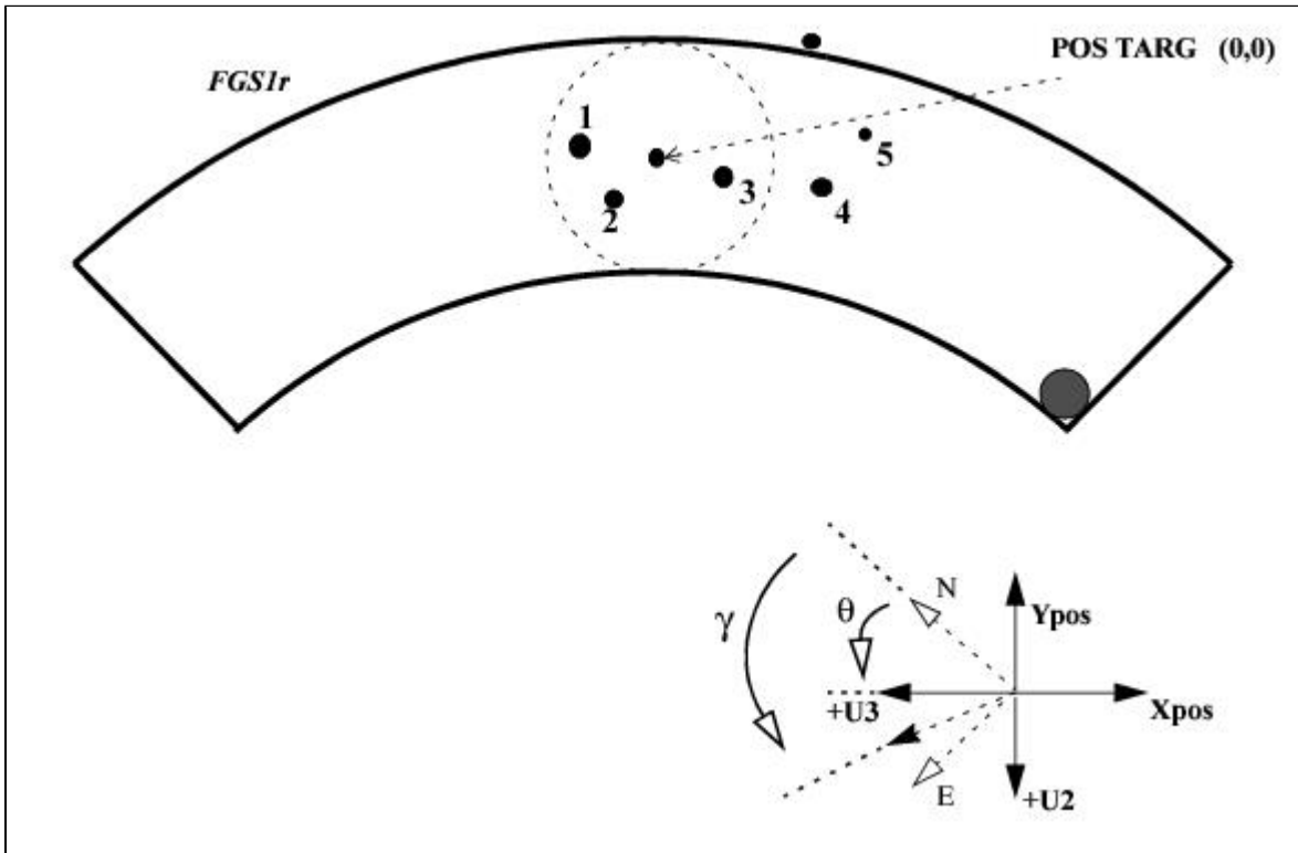
Figure 6.3: Example 3: Trans + Pos Mode Visits
