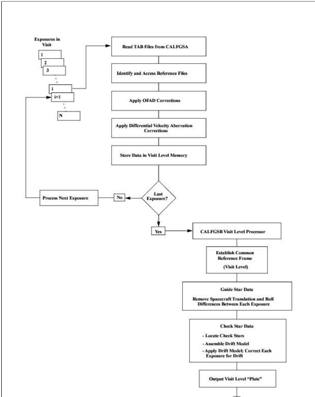
Figure 7.3: CALFGSB Position Mode Processing
