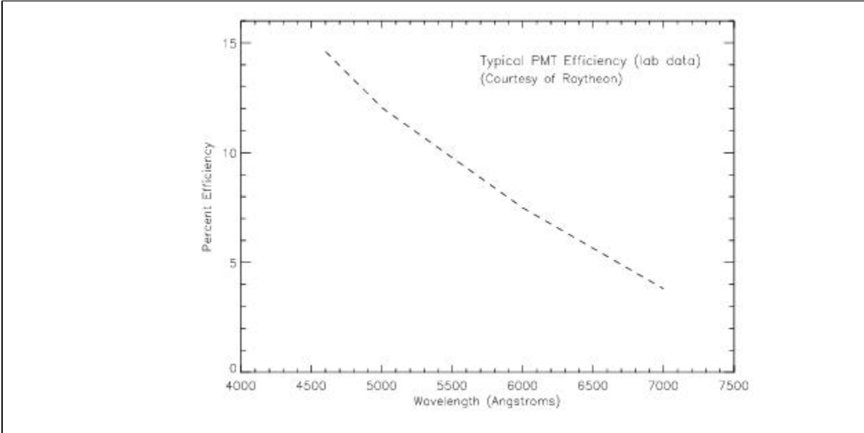
Figure 2.12: PMT Efficiency
