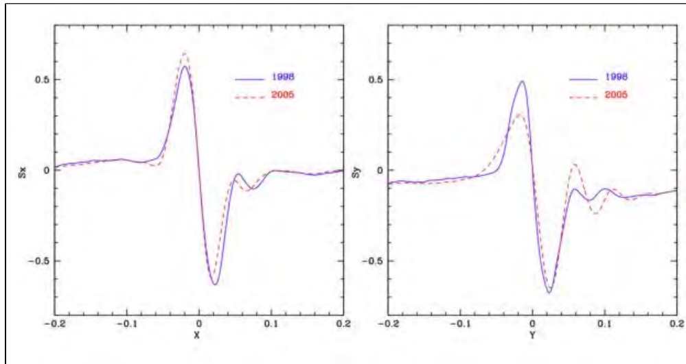
Figure 2.7:FGS1r S-curves
