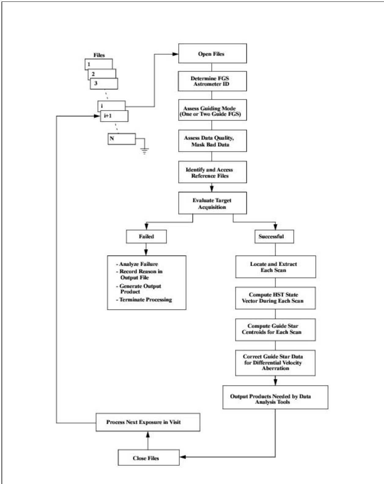
Figure 7.2: CALFGSA Transfer Mode Processing Tasks
