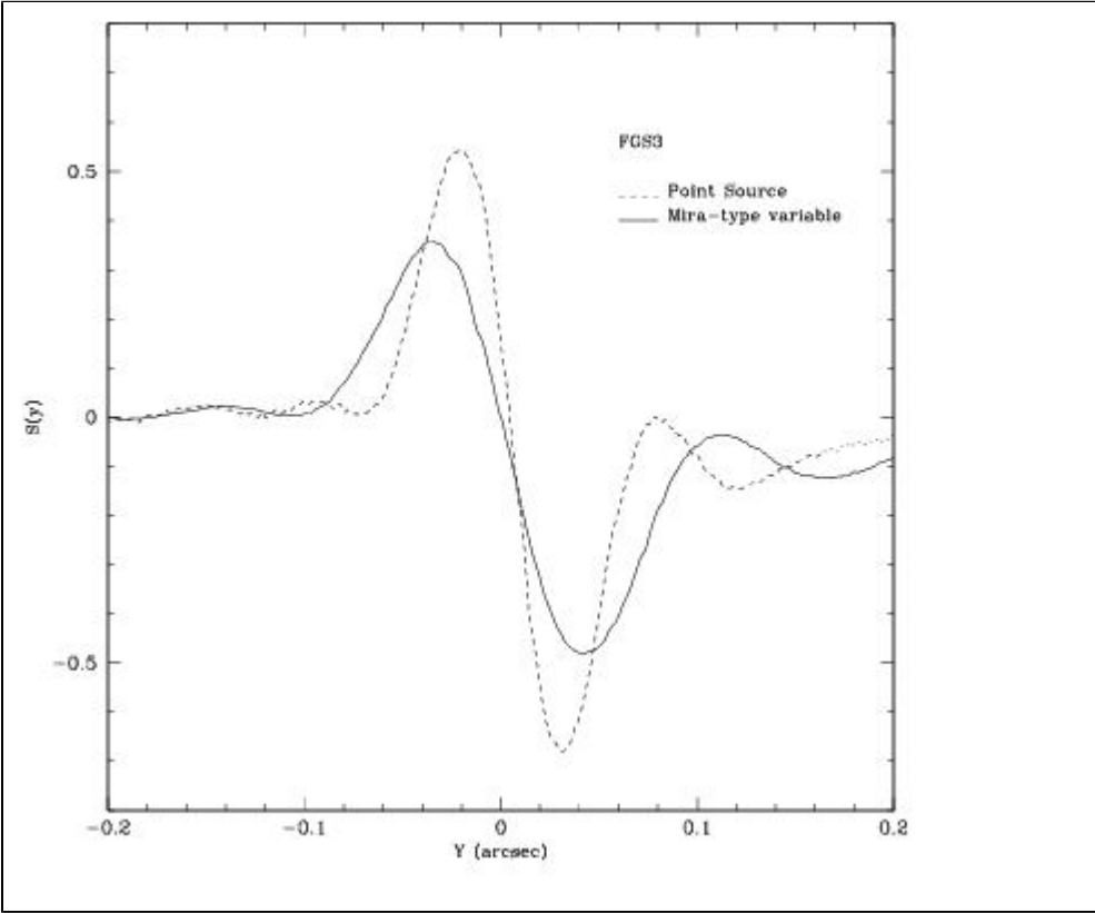
Figure 3.5: Mira-type variable with a resolved circumstellar disk
