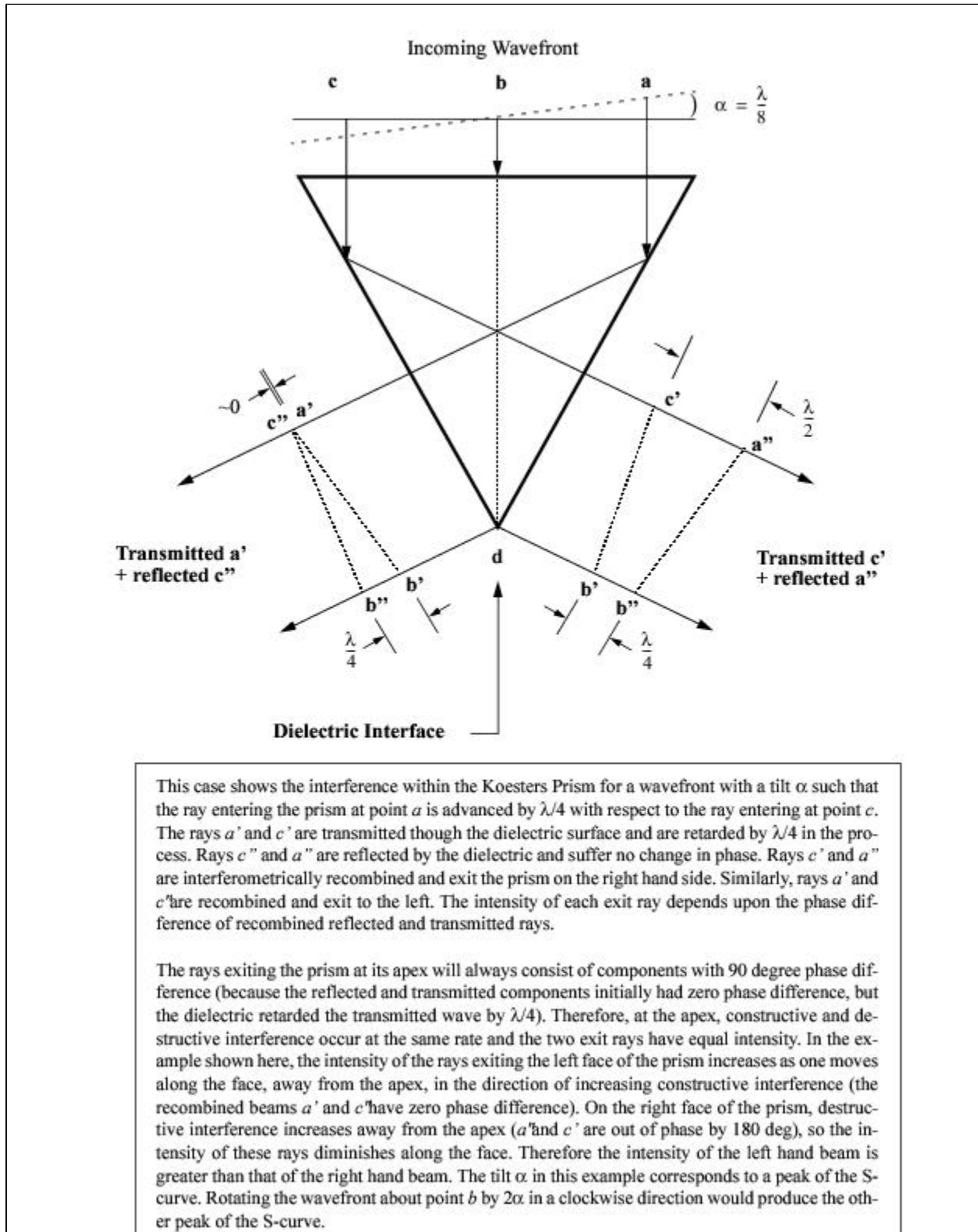
Figure 2.3: The Koesters Prism: Constructive and Destructive Interference.
