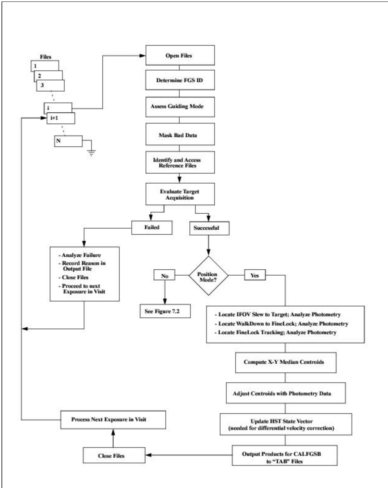
Figure 7.1: CALFGSA Common Processing Tasks
