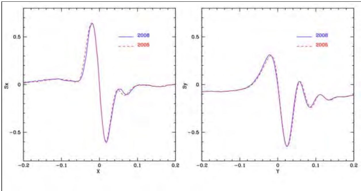
Figure 2.8: FGS1r S-curves 2005
