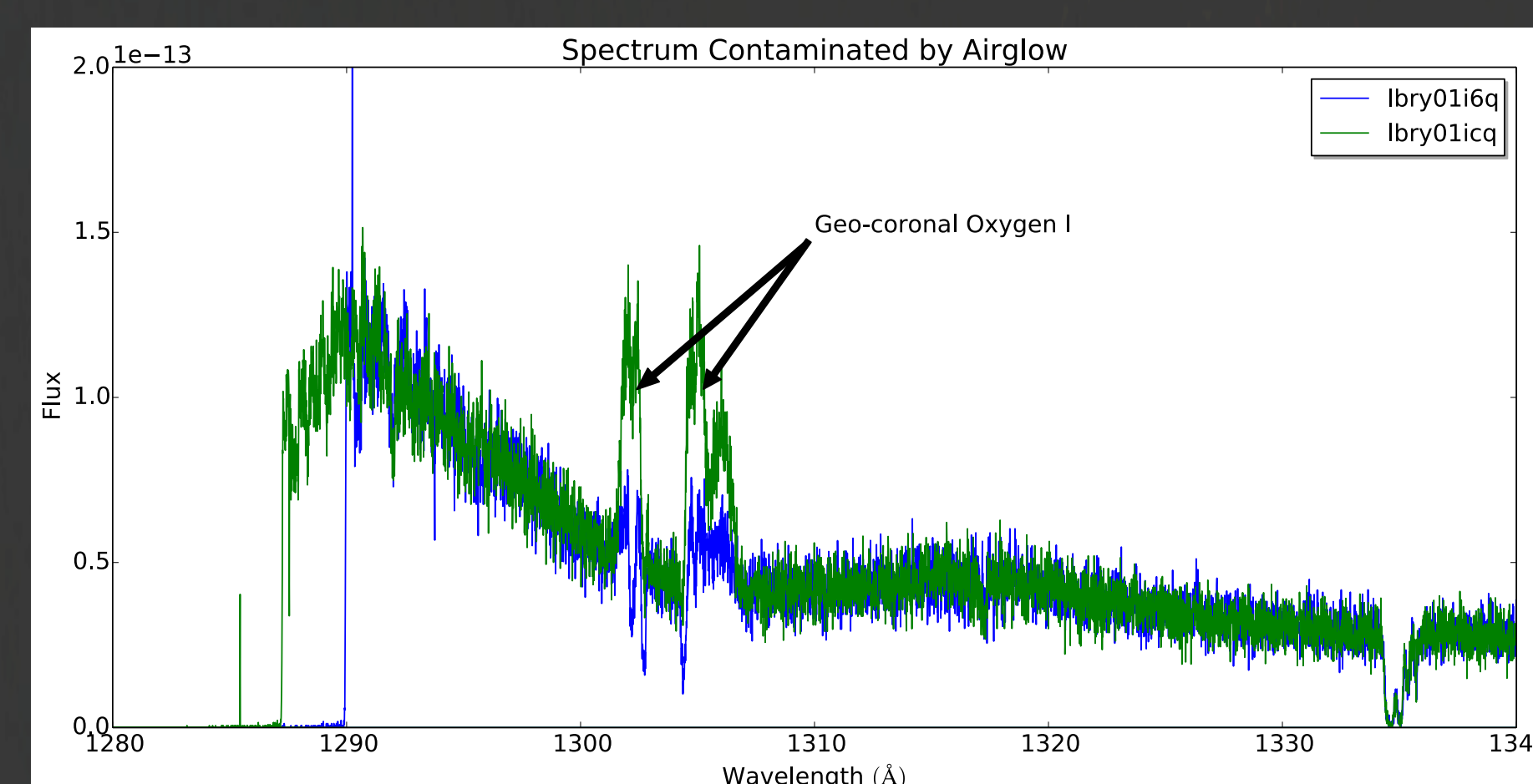
Figure 2 shows two COS x1d spectra as extracted by CalCOS. The variable emission features seen between 1300 and 1310 Angstroms are due to Oxygen I in the atmosphere at HST's orbit. Their presence in the spectrum can hide the presence of spectral features intrinsic to the source.
