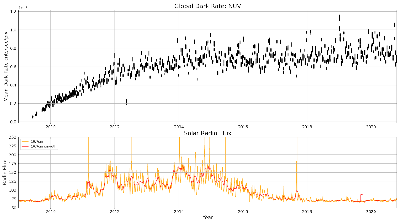
Figure 4. Dark Rate vs. Time: The COS NUV dark rate as a function of time through Cycle 27 prior to correcting the dark rate calculation. Similar to Figure4.
