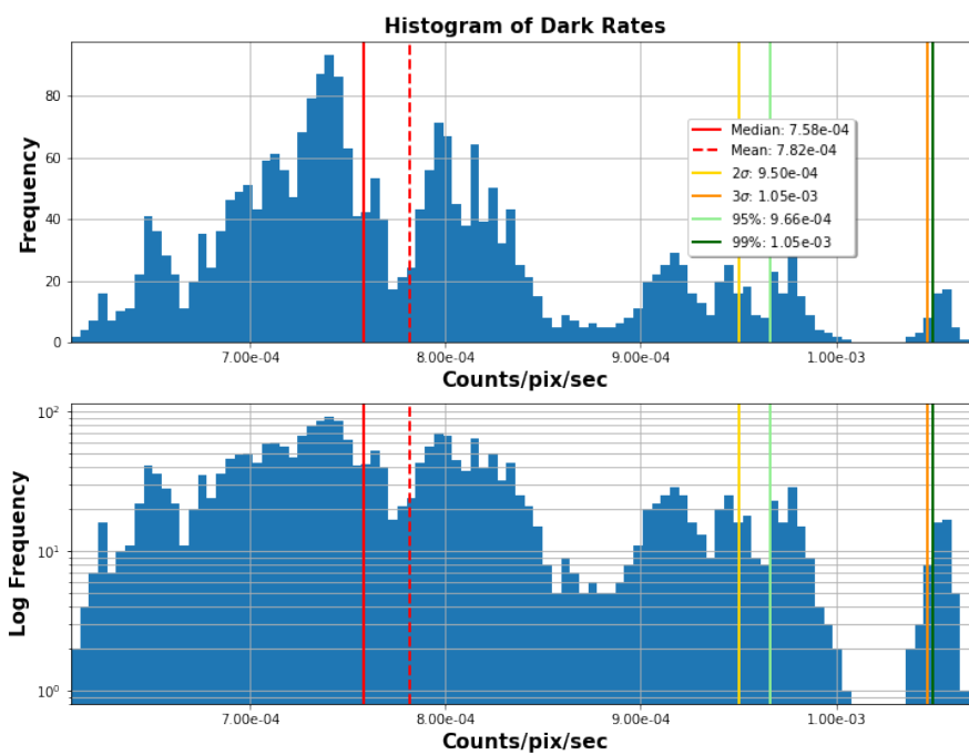
Figure 2. Dark Rate Distribution: The updated COS NUV dark rate from Cycle 27 prior to the correction, binned and then fit with a standard probability distribution to determine the value below which 95% of measured values fall
