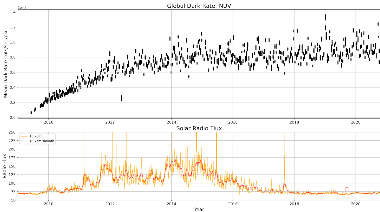
Figure 1. Dark Rate vs. Time: The updated COS NUV dark rate as a function of time, spanning from installation through Cycle 27. The dark rate is measured in 25 s increments, which is then plotted against the time in decimal year ( top ). Groupings of points occur naturally, as they correspond to the individual exposures of their origin, also displaying the natural variation within an exposure. We also plot these trends against the 10.7 cm radio flux, used as a signifier of the solar cycle ( bottom ).
