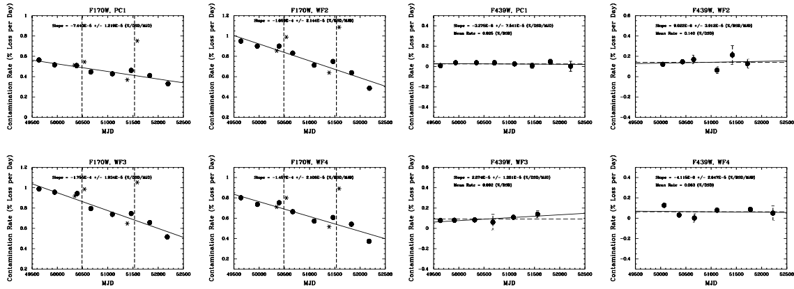
Figure 2. Fits to the contamination rates for F170W (left) and F439W (right). See McMaster & Whitmore (2002).
