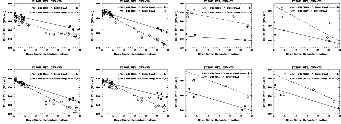
Figure 1. Contamination rates for 1997–1998 (open circles) and 2001–2002 (filled circles) for F170W (left) and F336W (right).
