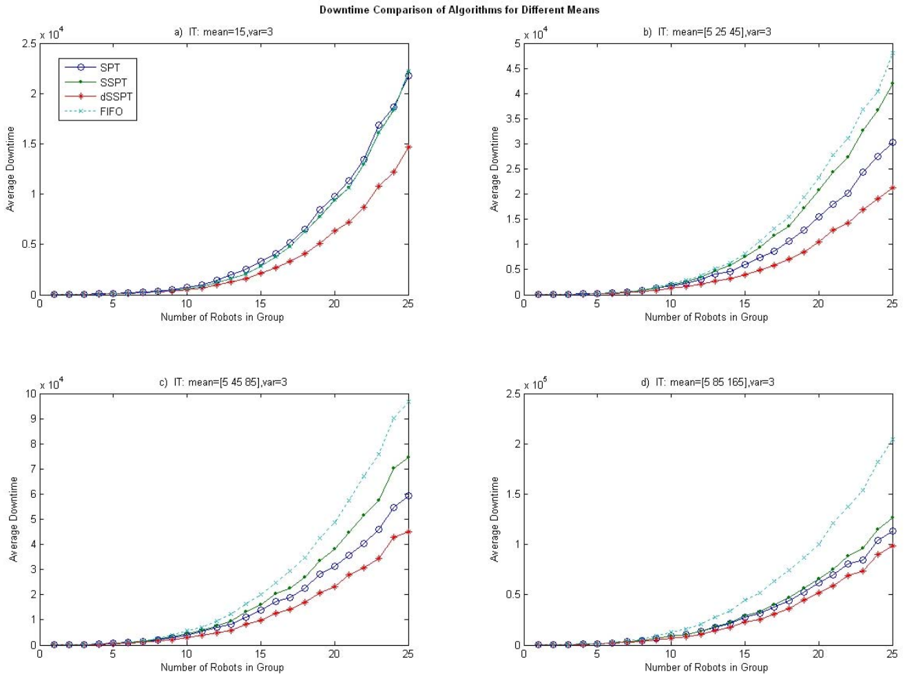
Figure 7: Downtime comparison for changing mean IT
