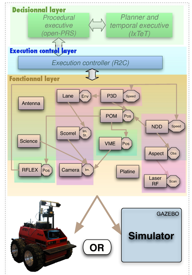
Figure 3: The LAAS architecture used for controlling the DALA mobile robot.
