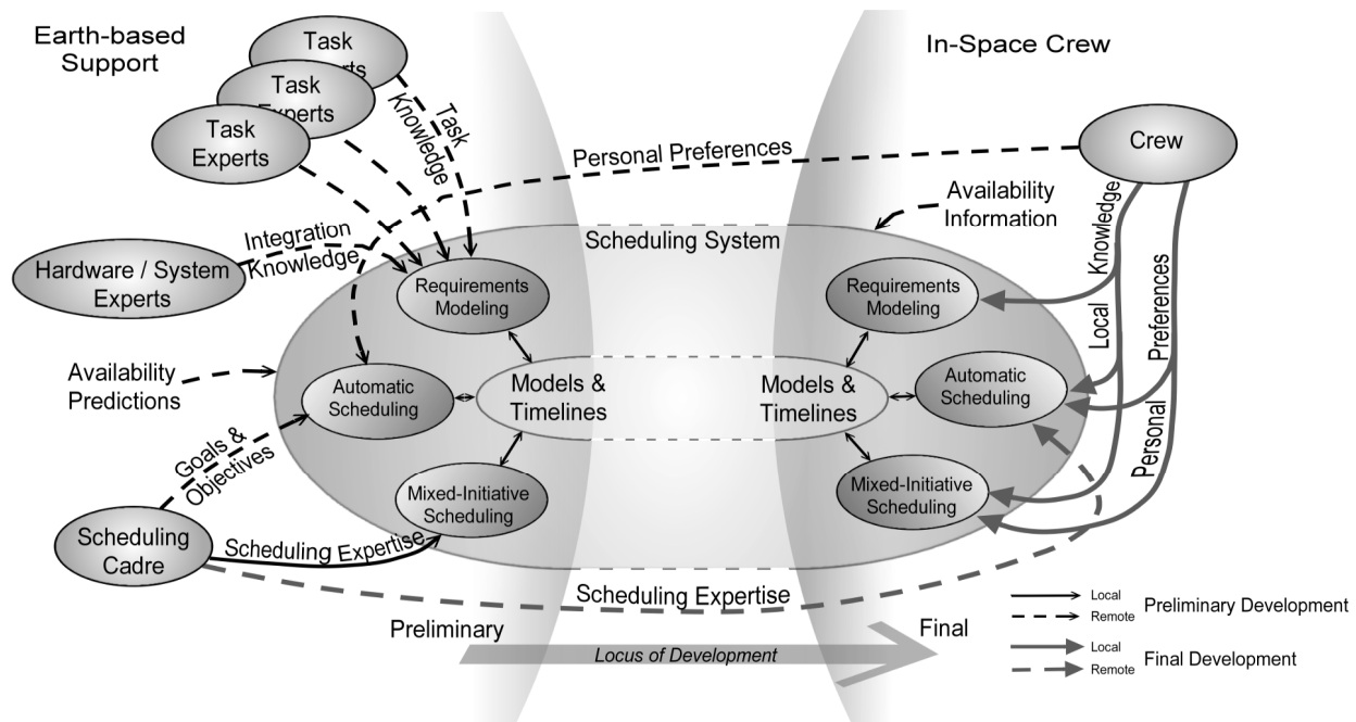
Figure 2. Concept of Operations
