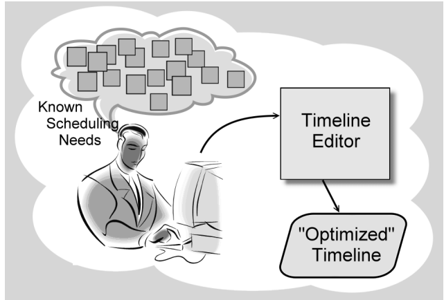
Figure 5. Mixed-Initiative Scheduling
