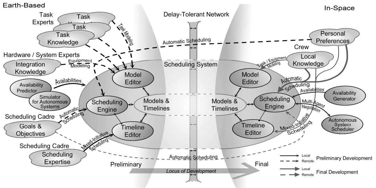
Figure 3. Software and Infrastructure
