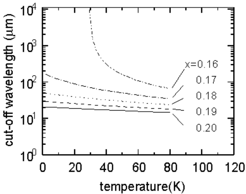
Fig.1: The cut-off wavelength is plotted against operating temperature for various composition values.
