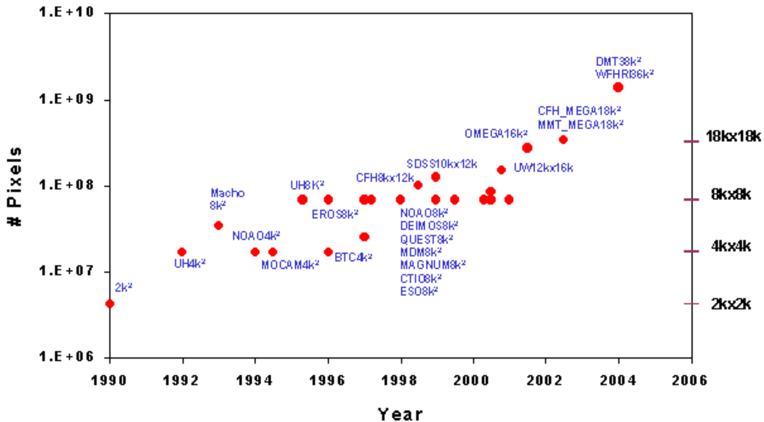
Figure 1: Plot showing the growth of focal plane arrays (total number of pixels), as a function of time, with current and planned flight CCD focal arrays. Penalty of a reduction in full well capacity of 50% to 70%, compared to a non-MPP device. MPP may also help mitigate the problem of hot pixels which appear as a result of radiation damage to CCDs, however, this remains to be experimentally demonstrated.
