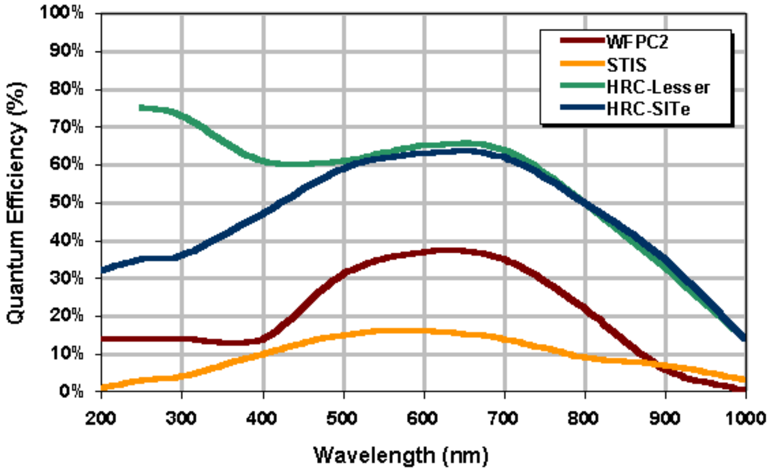
Figure 2: Visible QE curves obtained offered by several CCD vendors and laboratories, with the HST's Wide Field and Planetary Camera 2 (WFCP2) frontside-illuminated CCD shown for comparison.
