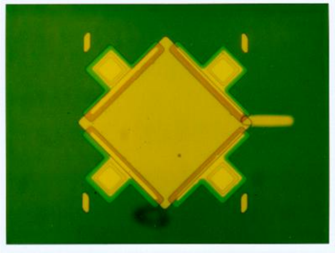
Fig 3 –Square absorber for x-y readout by four STJs, each of which has an Al trap as shown in Fig. 2. Device fabricated at Yale. Dimensions are 100 μm x 100 μm for the square. Tests of similar structures have been done at ESA [7].
