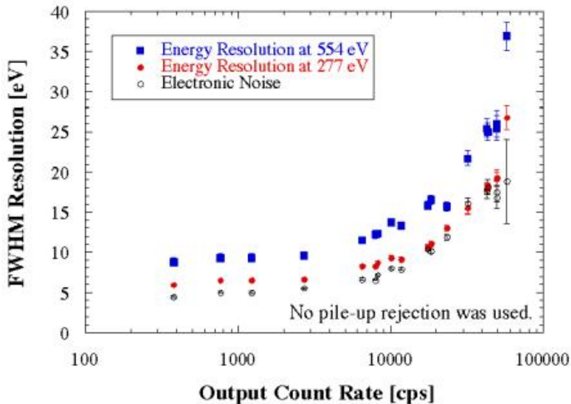
Fig 5. Energy width vs. count rate, from S. Friedrich for the Livermore Lab group "Energy resolution and high count rate performance of superconducting tunnel junction x-ray spectrometers", M. Frank, L.J. Hiller, J.B. LeGrand, C.A. Mears, S.E. Labov, M.A. Lindeman, H. Netel, D. Chow, A.T. Barfknecht, Rev. Sci. Instr. 69, 25 (1998)
