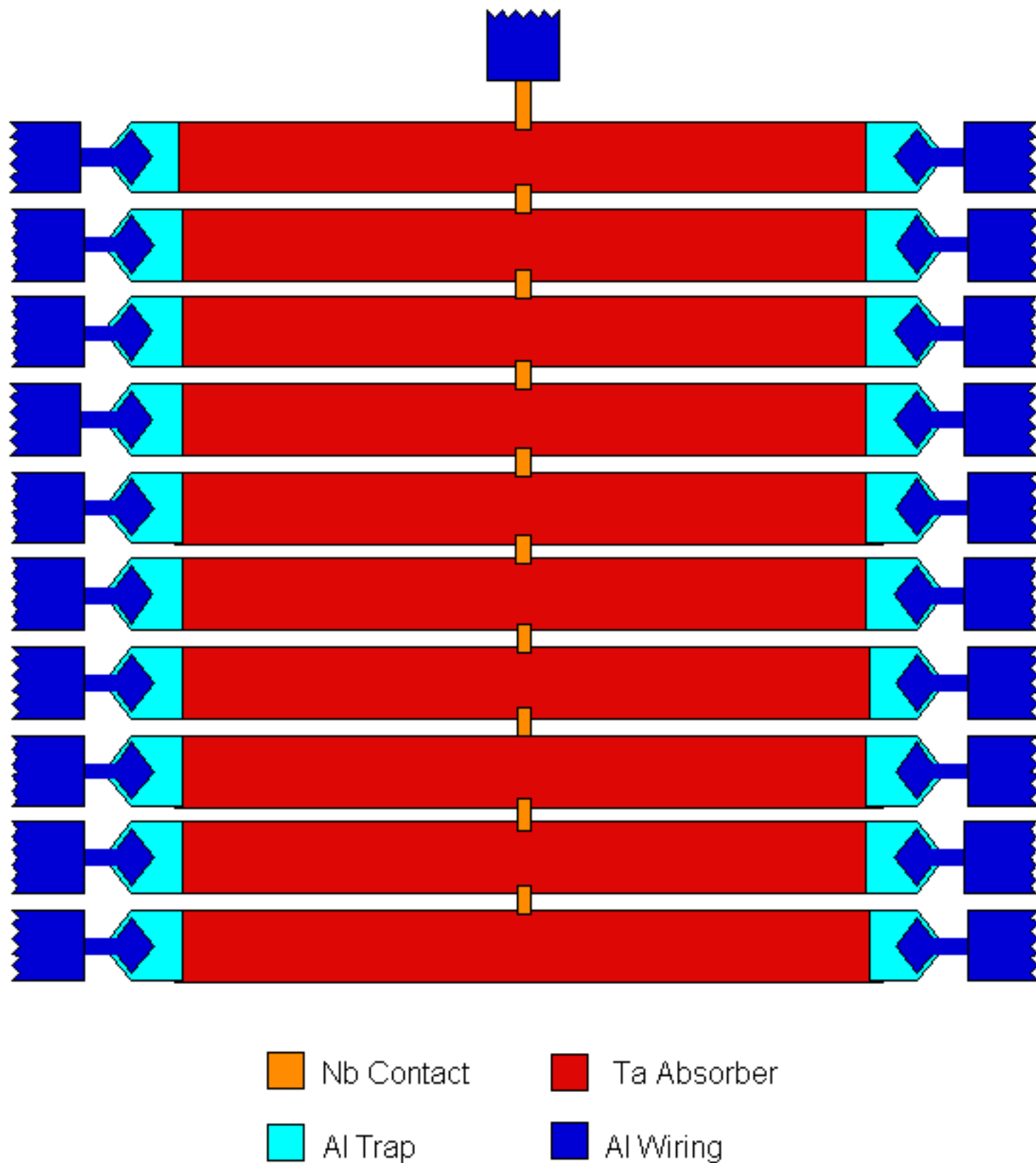
Fig. 7 Proposed 450 pixel camera design, for use on the Palomar 200 inch telescope. The first design will use a cold FET readout of each STJ, and achieve E/DEH 45 at E = 5 eV. An imaging fiber bundle will provide coverage in the visible into the near-UV. (C. Wilson, D.Prober, D.Schiminovich, and C. Martin, unpublished)
