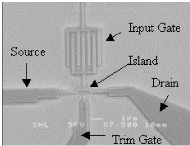
Figure 1. SET with input gate.
