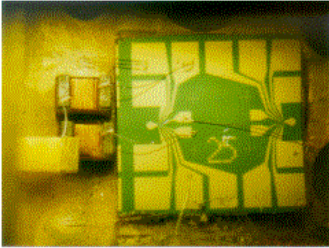
Figure 3. Two-channel WDM with SETs, inductors, and coaxial launcher wirebonded together. Chip is 7 mm square; SETs are at confluence of optical traces.
