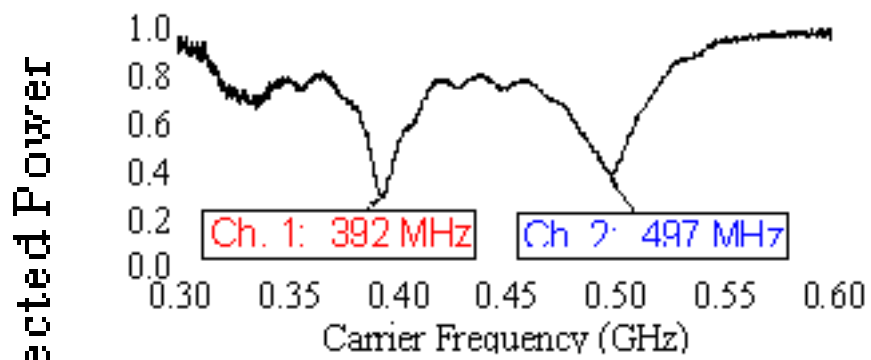
Figure 4. Reflected power versus frequency shows resonance frequencies for two parallel RF-SET tank circuits.
