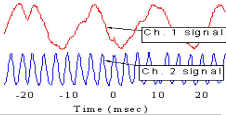
Figure 5. De-multiplexed signals from the two RF-SETs.
