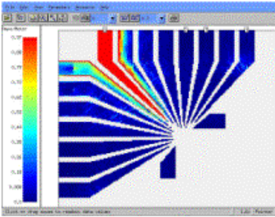
Figure 7. Charge density for cross capacitance calculation: voltage on one pad induces charges on all.
