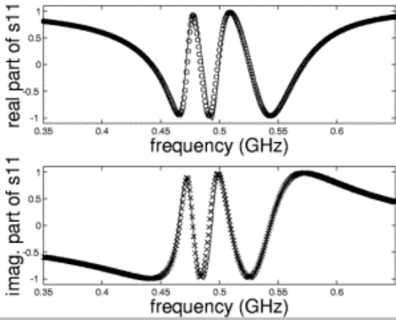
Figure 8. Reflection coefficient for three tank circuit array. Data (points) and parametric model (curves).
