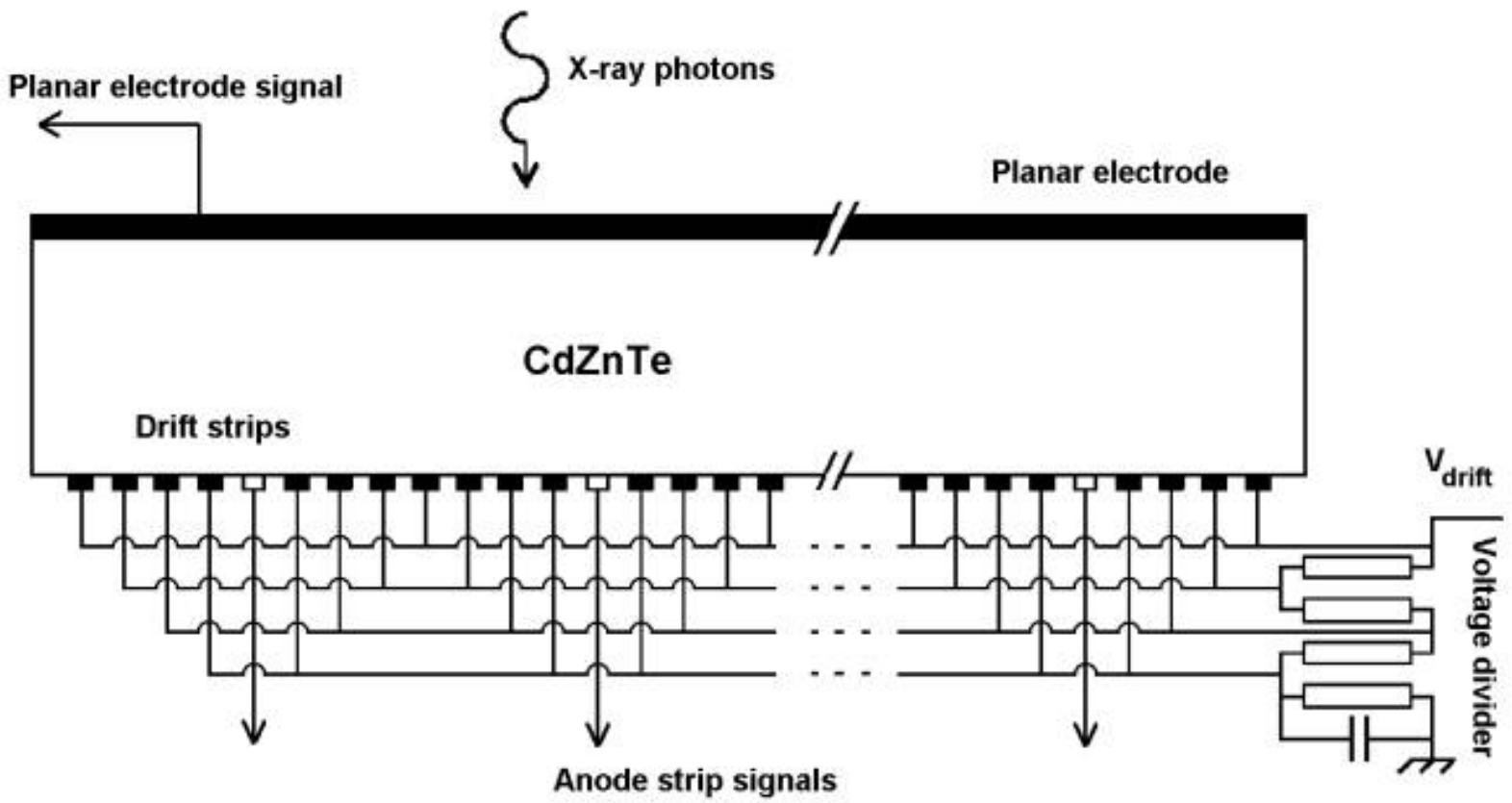
Figure 1. Cross-section of a detector based on the drift-strip method. The drift-strip electrodes are biased such a way that the negative charge carriers (electrons) move to the anode strips.
